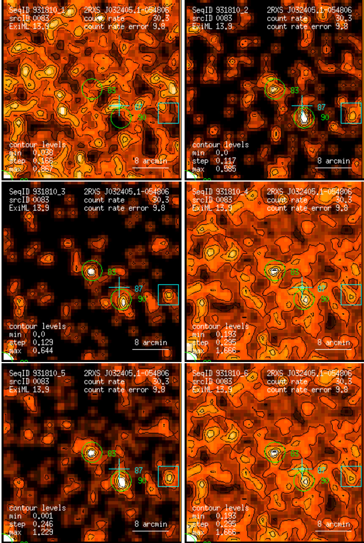
Figure 83: RASS 931810: detection 0083: band rate images, Gaussian filter: (1) PSPC channels 11 – 41, (2) 52 – 90, (3) 91 – 201, (4) 11 – 235, (5) 52 – 201, (6) 11 – 201. Broad band rates in counts/ks. Band rate contour levels in counts/ks/arcmin 2 .
