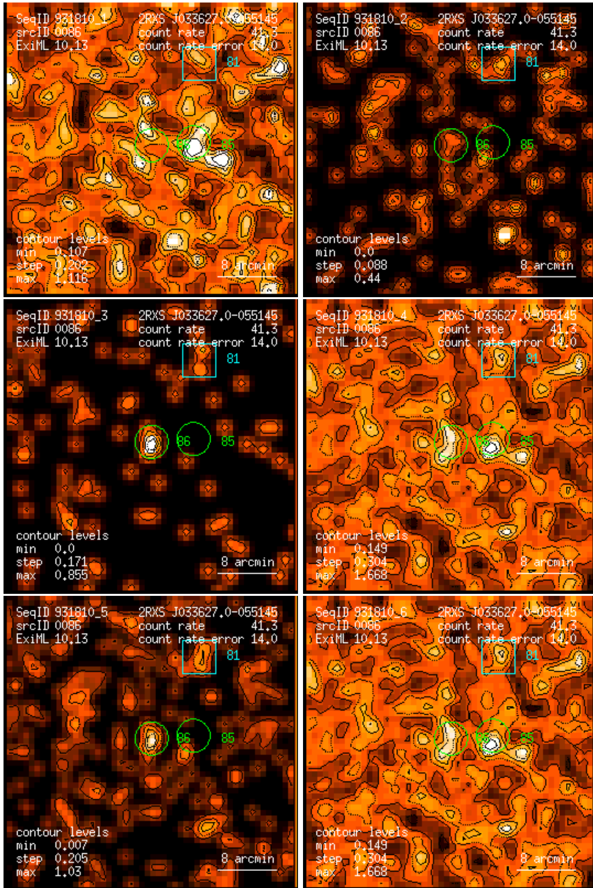
Figure 86: RASS 931810: detection 0086: band rate images, Gaussian filter: (1) PSPC channels 11 – 41, (2) 52 – 90, (3) 91 – 201, (4) 11 – 235, (5) 52 – 201, (6) 11 – 201. Broad band rates in counts/ks. Band rate contour levels in counts/ks/arcmin 2 .
