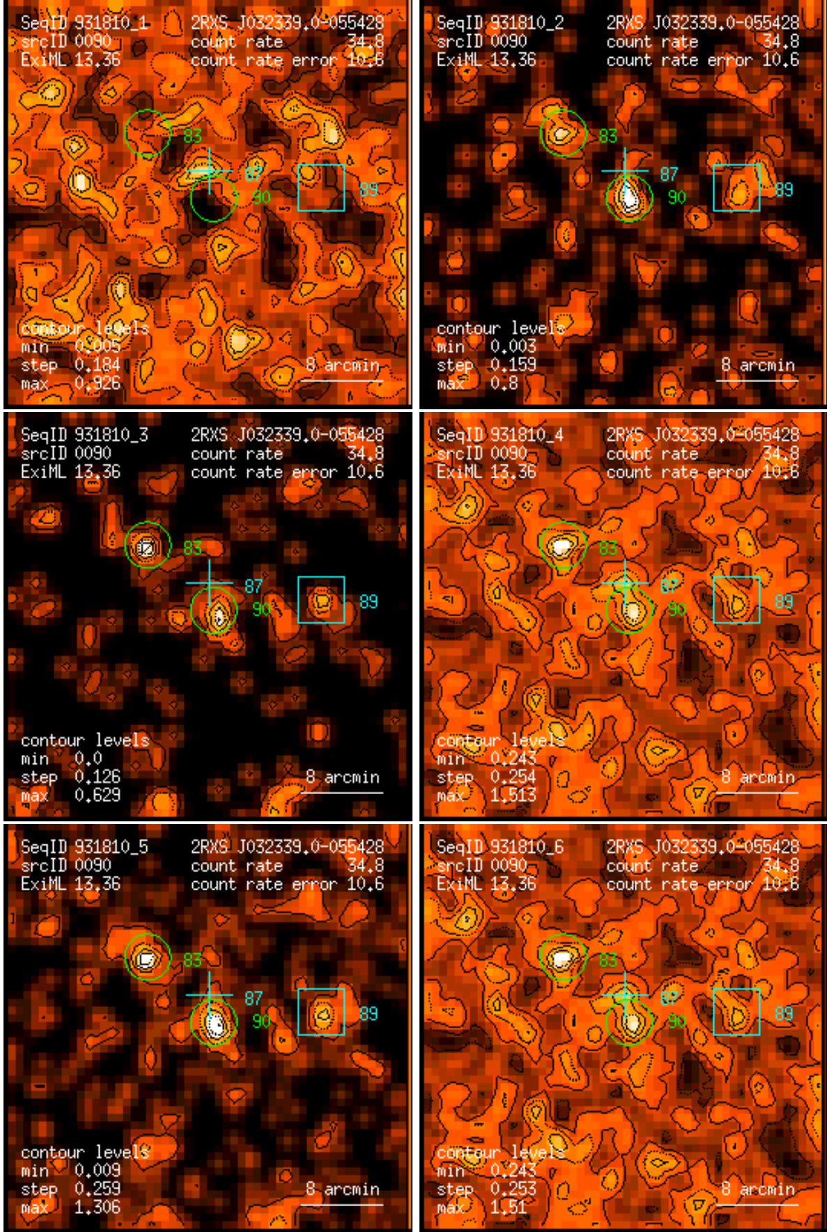
Figure 90: RASS 931810: detection 0090: band rate images, Gaussian filter: (1) PSPC channels 11 – 41, (2) 52 – 90, (3) 91 – 201, (4) 11 – 235, (5) 52 – 201, (6) 11 – 201. Broad band rates in counts/ks. Band rate contour levels in counts/ks/arcmin 2 .
