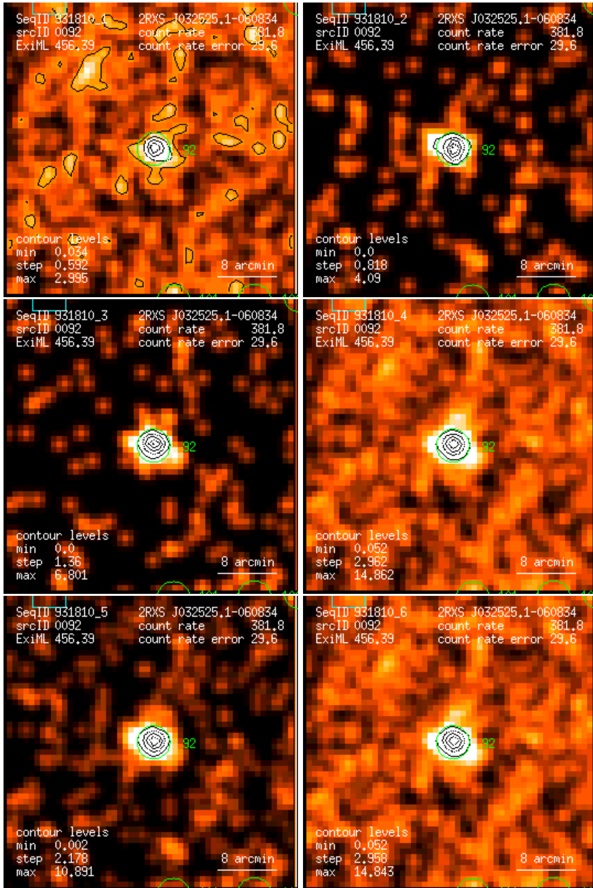
Figure 92: RASS 931810: detection 0092: band rate images, Gaussian filter: (1) PSPC channels 11 – 41, (2) 52 – 90, (3) 91 – 201, (4) 11 – 235, (5) 52 – 201, (6) 11 – 201. Broad band rates in counts/ks. Band rate contour levels in counts/ks/arcmin 2 .
