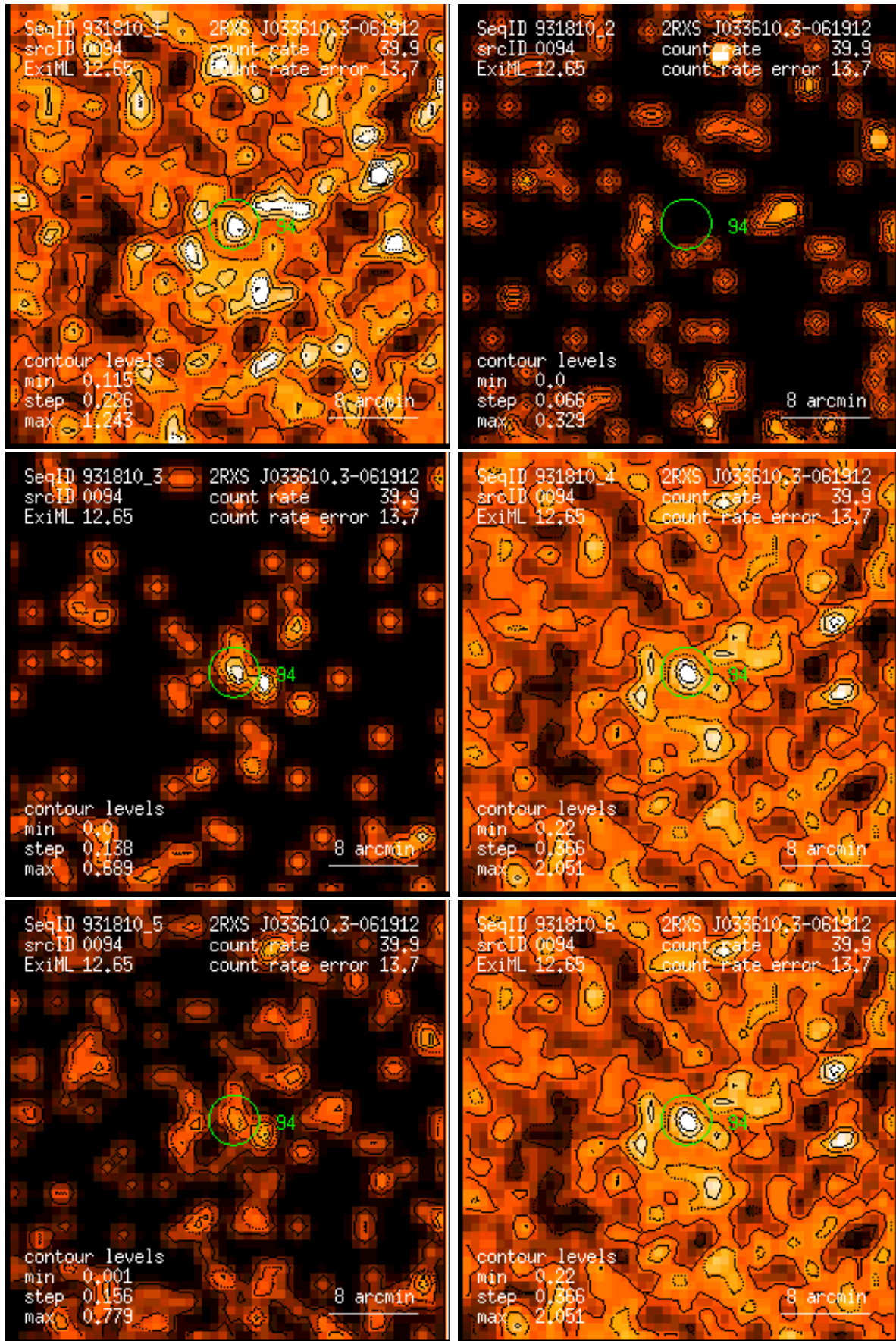
Figure 94: RASS 931810: detection 0094: band rate images, Gaussian filter: (1) PSPC channels 11 – 41, (2) 52 – 90, (3) 91 – 201, (4) 11 – 235, (5) 52 – 201, (6) 11 – 201. Broad band rates in counts/ks. Band rate contour levels in counts/ks/arcmin 2 .
