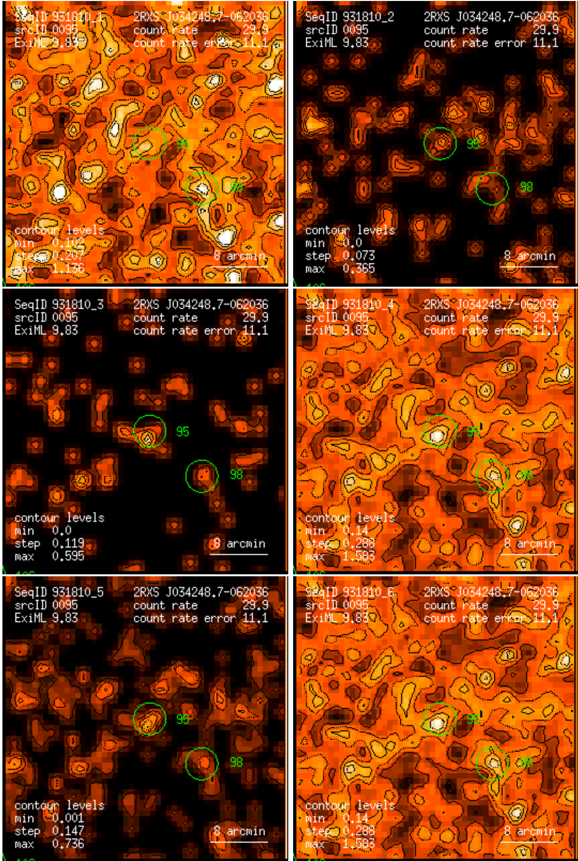
Figure 95: RASS 931810: detection 0095: band rate images, Gaussian filter: (1) PSPC channels 11 – 41, (2) 52 – 90, (3) 91 – 201, (4) 11 – 235, (5) 52 – 201, (6) 11 – 201. Broad band rates in counts/ks. Band rate contour levels in counts/ks/arcmin 2 .
