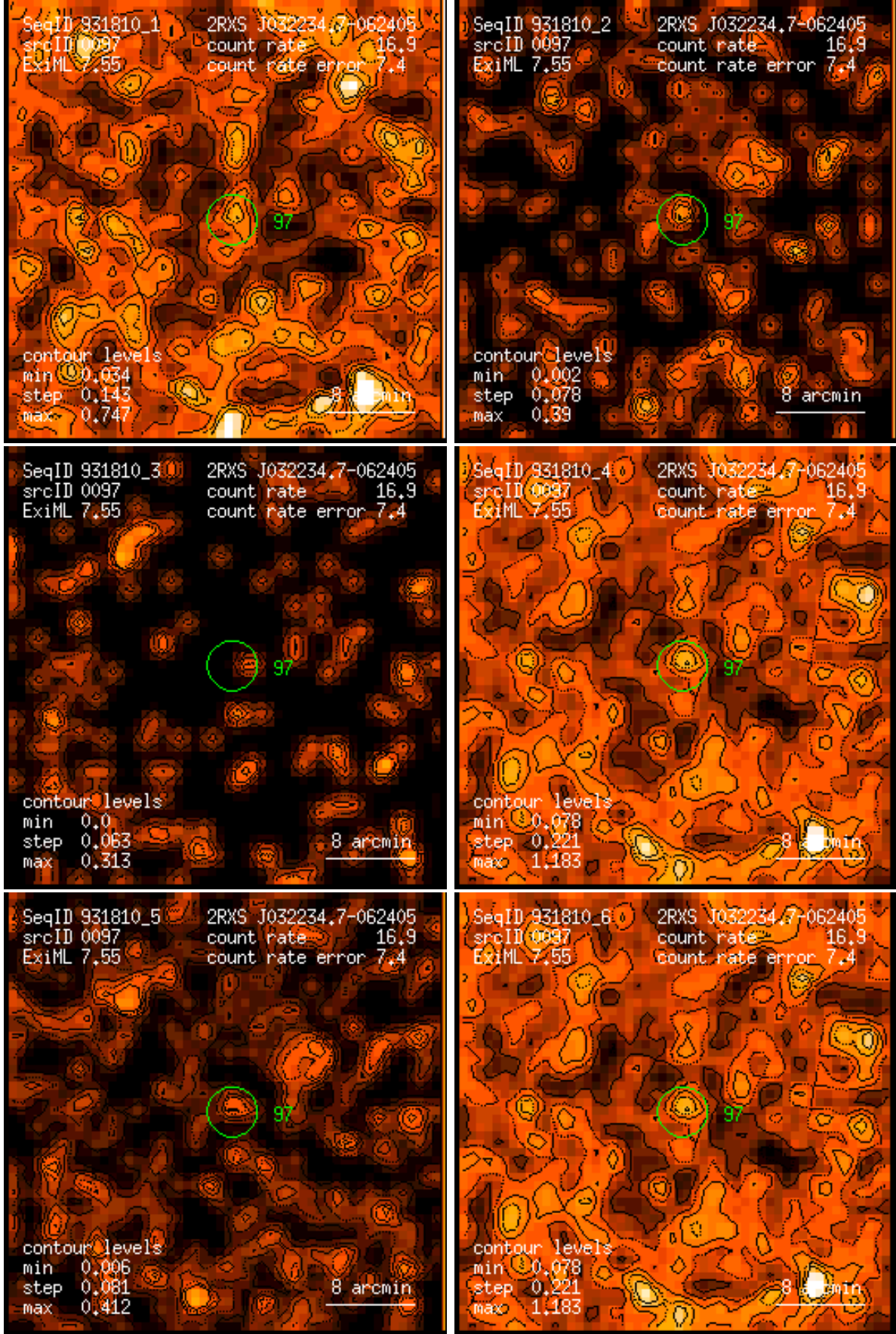
Figure 97: RASS 931810: detection 0097: band rate images, Gaussian filter: (1) PSPC channels 11 – 41, (2) 52 – 90, (3) 91 – 201, (4) 11 – 235, (5) 52 – 201, (6) 11 – 201. Broad band rates in counts/ks. Band rate contour levels in counts/ks/arcmin 2 .
