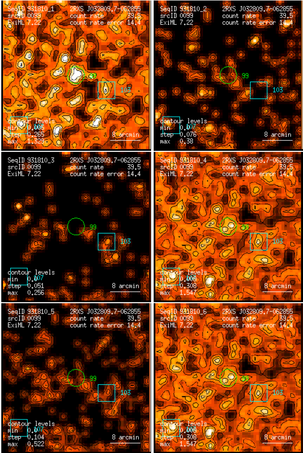
Figure 99: RASS 931810: detection 0099: band rate images, Gaussian filter: (1) PSPC channels 11 – 41, (2) 52 – 90, (3) 91 – 201, (4) 11 – 235, (5) 52 – 201, (6) 11 – 201. Broad band rates in counts/ks. Band rate contour levels in counts/ks/arcmin 2 .
