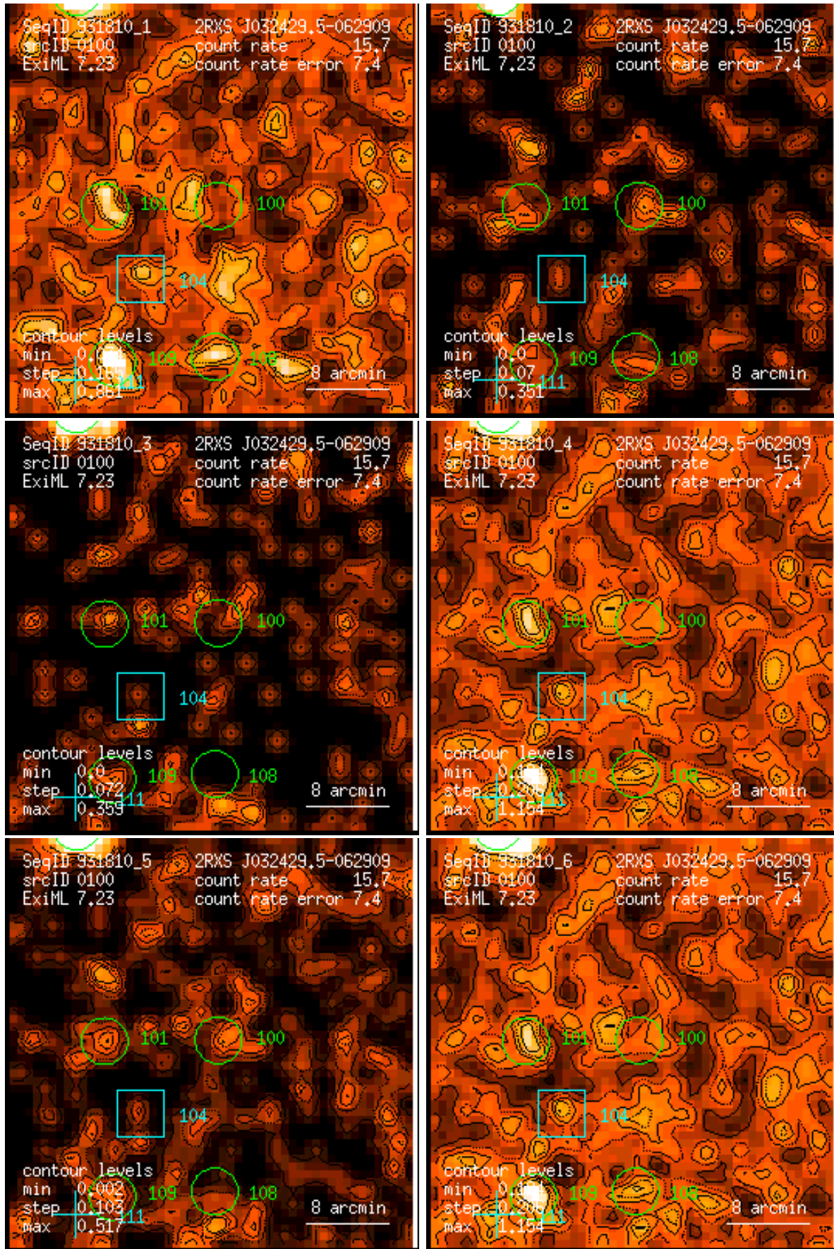
Figure 100: RASS 931810: detection 0100: band rate images, Gaussian filter: (1) PSPC channels 11 – 41, (2) 52 – 90, (3) 91 – 201, (4) 11 – 235, (5) 52 – 201, (6) 11 – 201. Broad band rates in counts/ks. Band rate contour levels in counts/ks/arcmin 2 .
