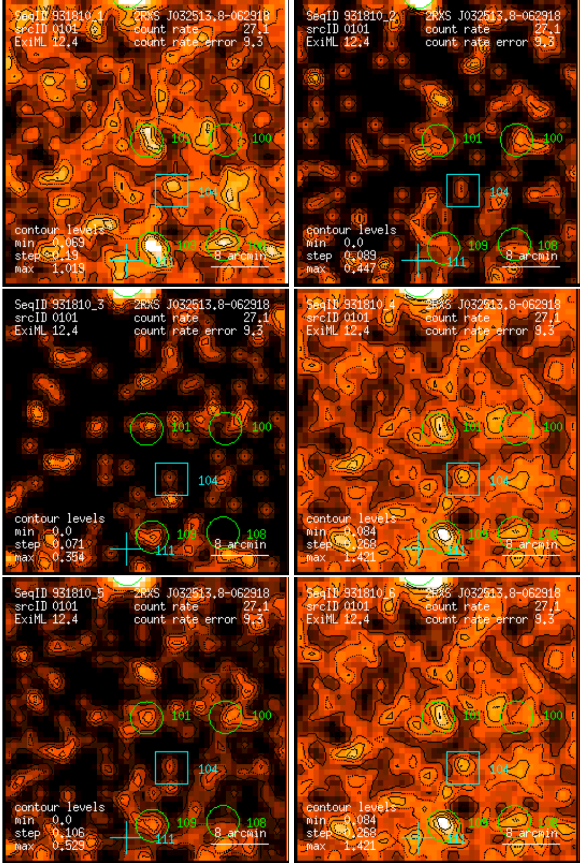
Figure 101: RASS 931810: detection 0101: band rate images, Gaussian filter: (1) PSPC channels 11 – 41, (2) 52 – 90, (3) 91 – 201, (4) 11 – 235, (5) 52 – 201, (6) 11 – 201. Broad band rates in counts/ks. Band rate contour levels in counts/ks/arcmin 2 .
