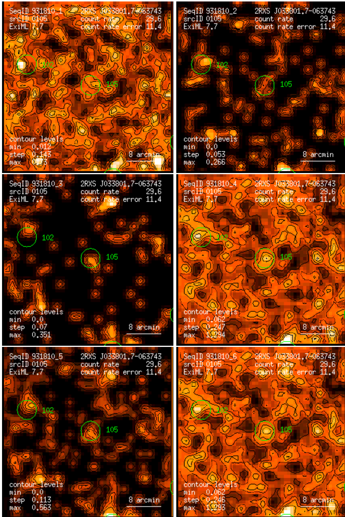
Figure 105: RASS 931810: detection 0105: band rate images, Gaussian filter: (1) PSPC channels 11 – 41, (2) 52 – 90, (3) 91 – 201, (4) 11 – 235, (5) 52 – 201, (6) 11 – 201. Broad band rates in counts/ks. Band rate contour levels in counts/ks/arcmin 2 .
