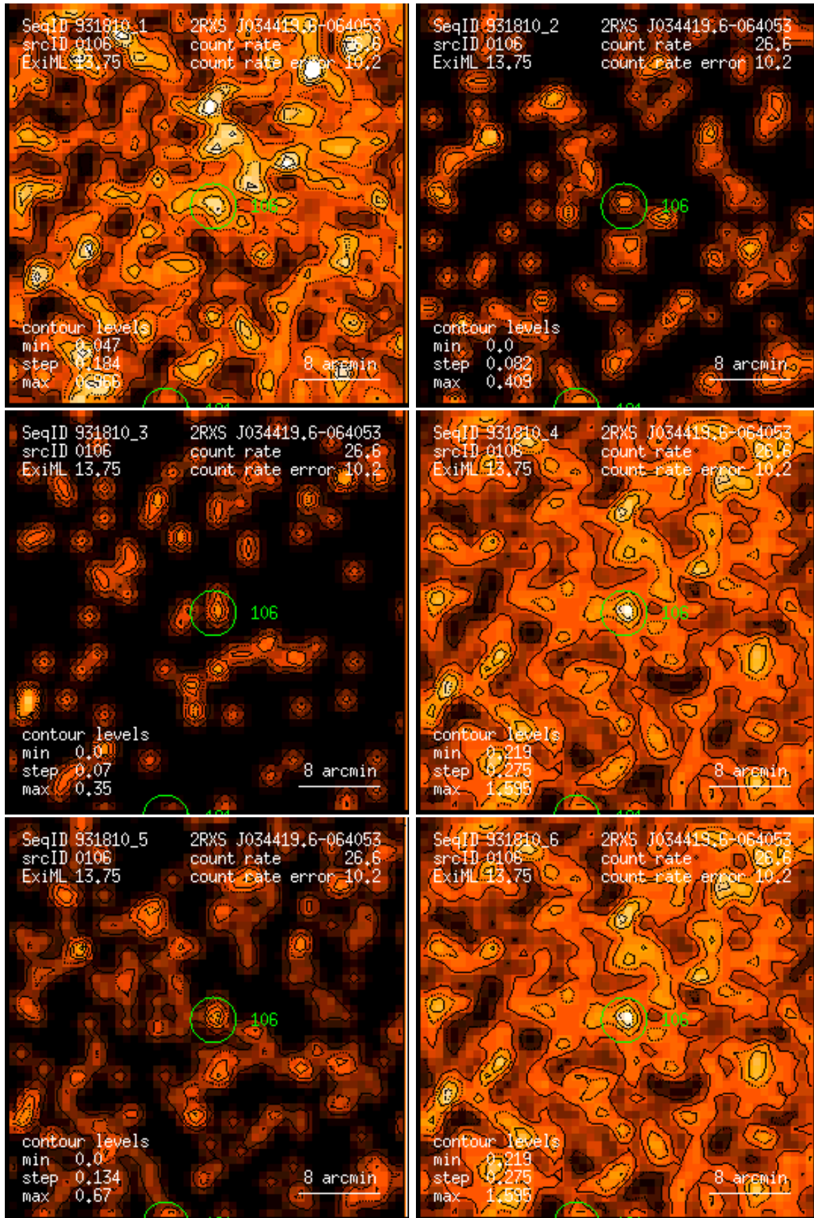
Figure 106: RASS 931810: detection 0106: band rate images, Gaussian filter: (1) PSPC channels 11 – 41, (2) 52 – 90, (3) 91 – 201, (4) 11 – 235, (5) 52 – 201, (6) 11 – 201. Broad band rates in counts/ks. Band rate contour levels in counts/ks/arcmin 2 .
