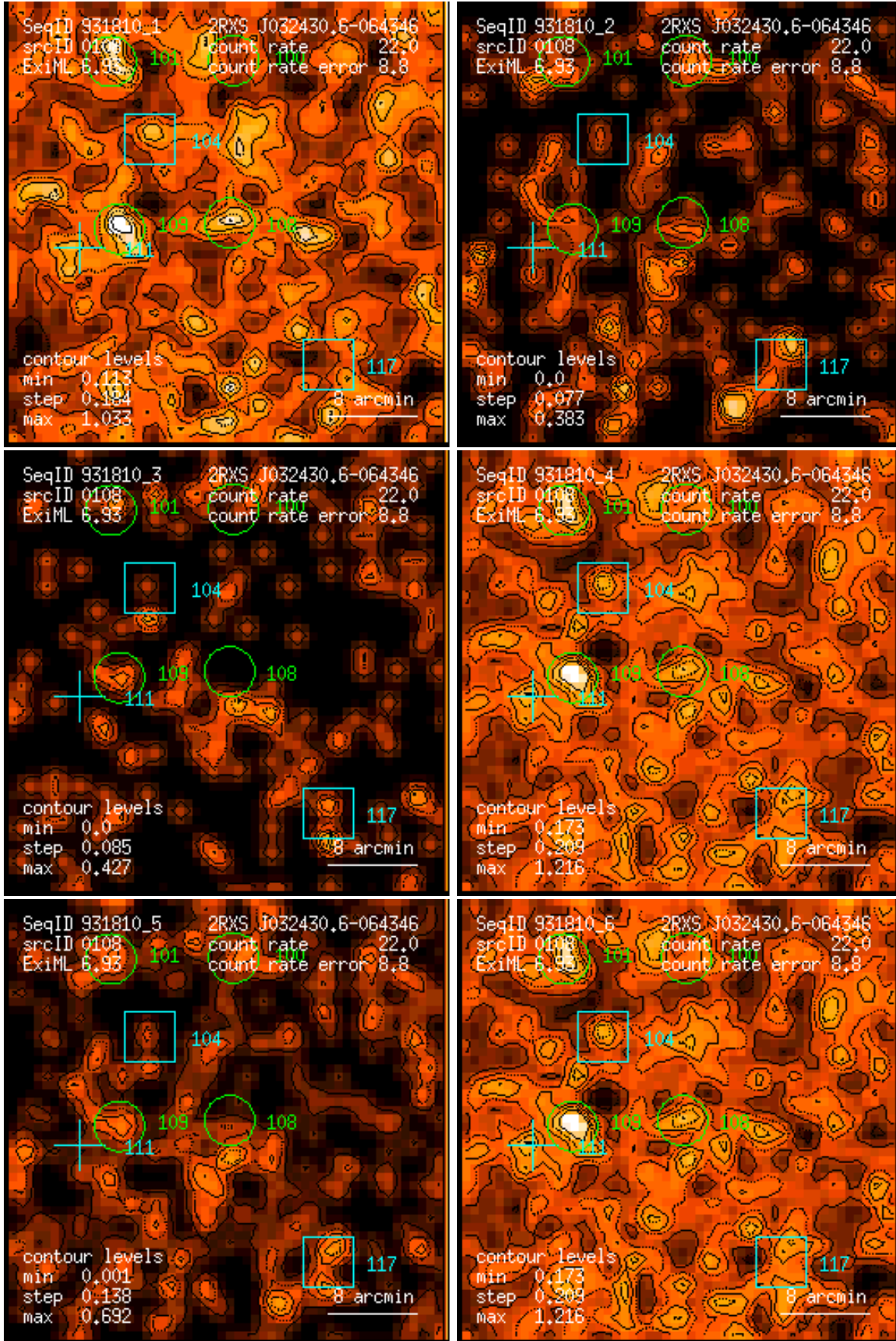
Figure 108: RASS 931810: detection 0108: band rate images, Gaussian filter: (1) PSPC channels 11 – 41, (2) 52 – 90, (3) 91 – 201, (4) 11 – 235, (5) 52 – 201, (6) 11 – 201. Broad band rates in counts/ks. Band rate contour levels in counts/ks/arcmin 2 .
