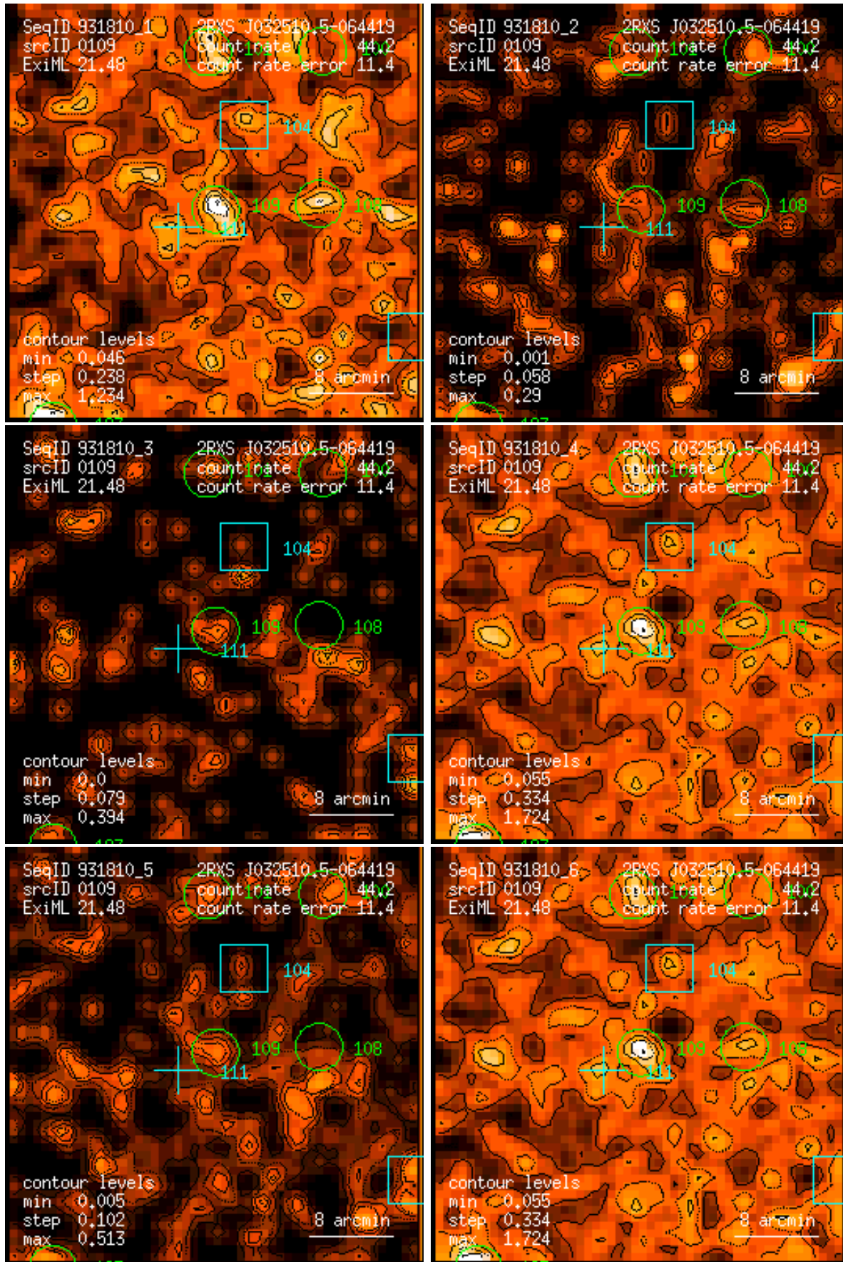
Figure 109: RASS 931810: detection 0109: band rate images, Gaussian filter: (1) PSPC channels 11 – 41, (2) 52 – 90, (3) 91 – 201, (4) 11 – 235, (5) 52 – 201, (6) 11 – 201. Broad band rates in counts/ks. Band rate contour levels in counts/ks/arcmin 2 .
