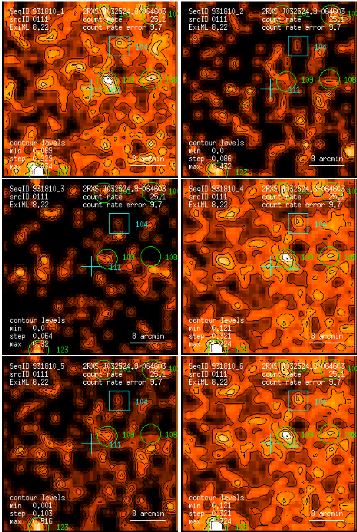
Figure 111: RASS 931810: detection 0111: band rate images, Gaussian filter: (1) PSPC channels 11 – 41, (2) 52 – 90, (3) 91 – 201, (4) 11 – 235, (5) 52 – 201, (6) 11 – 201. Broad band rates in counts/ks. Band rate contour levels in counts/ks/arcmin 2 .
