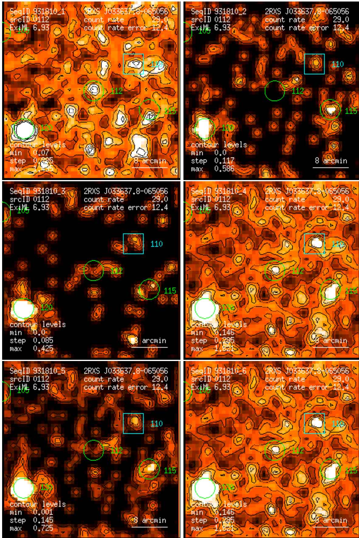
Figure 112: RASS 931810: detection 0112: band rate images, Gaussian filter: (1) PSPC channels 11 – 41, (2) 52 – 90, (3) 91 – 201, (4) 11 – 235, (5) 52 – 201, (6) 11 – 201. Broad band rates in counts/ks. Band rate contour levels in counts/ks/arcmin 2 .
