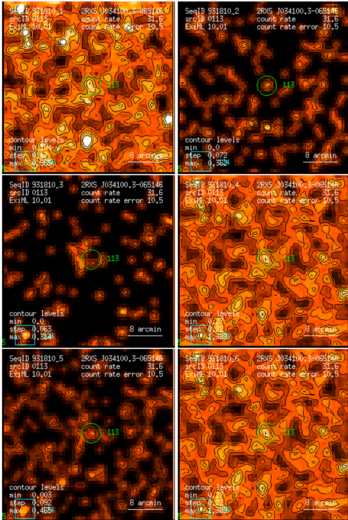
Figure 113: RASS 931810: detection 0113: band rate images, Gaussian filter: (1) PSPC channels 11 – 41, (2) 52 – 90, (3) 91 – 201, (4) 11 – 235, (5) 52 – 201, (6) 11 – 201. Broad band rates in counts/ks. Band rate contour levels in counts/ks/arcmin 2 .
