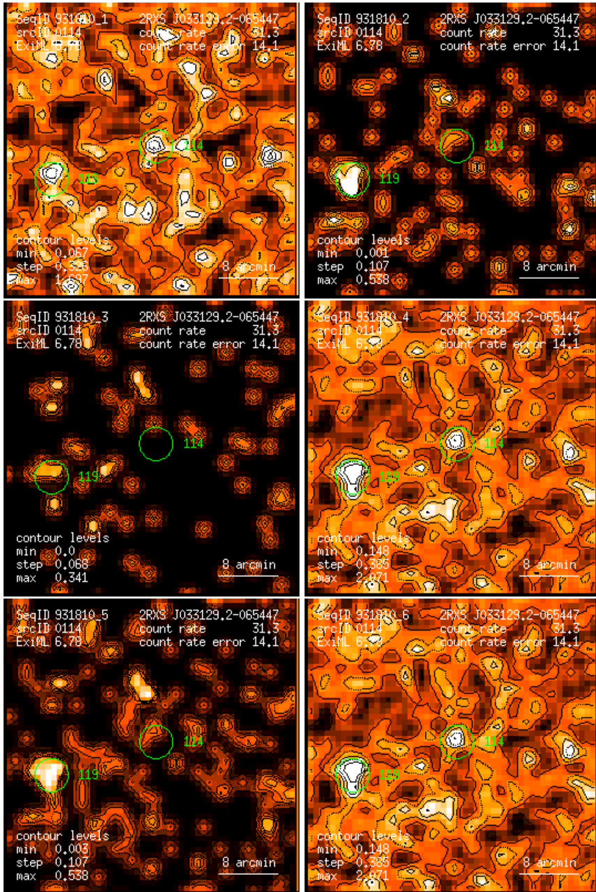
Figure 114: RASS 931810: detection 0114: band rate images, Gaussian filter: (1) PSPC channels 11 – 41, (2) 52 – 90, (3) 91 – 201, (4) 11 – 235, (5) 52 – 201, (6) 11 – 201. Broad band rates in counts/ks. Band rate contour levels in counts/ks/arcmin 2 .
