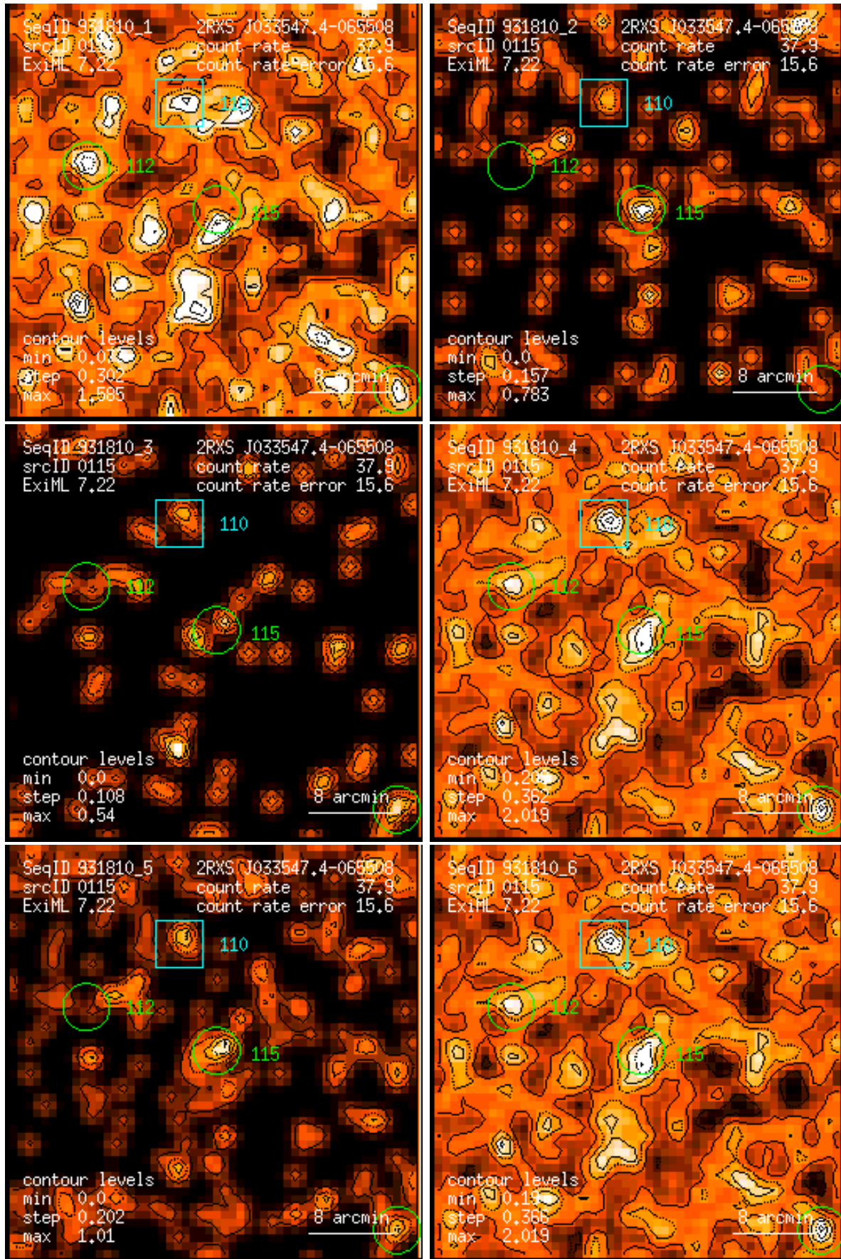
Figure 115: RASS 931810: detection 0115: band rate images, Gaussian filter: (1) PSPC channels 11 – 41, (2) 52 – 90, (3) 91 – 201, (4) 11 – 235, (5) 52 – 201, (6) 11 – 201. Broad band rates in counts/ks. Band rate contour levels in counts/ks/arcmin 2 .
