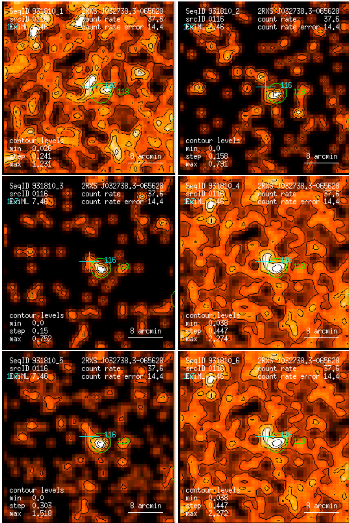
Figure 116: RASS 931810: detection 0116: band rate images, Gaussian filter: (1) PSPC channels 11 – 41, (2) 52 – 90, (3) 91 – 201, (4) 11 – 235, (5) 52 – 201, (6) 11 – 201. Broad band rates in counts/ks. Band rate contour levels in counts/ks/arcmin 2 .
