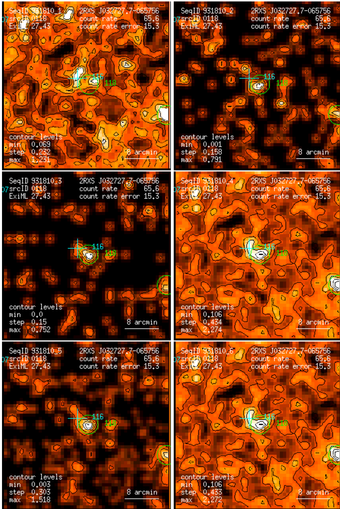
Figure 118: RASS 931810: detection 0118: band rate images, Gaussian filter: (1) PSPC channels 11 – 41, (2) 52 – 90, (3) 91 – 201, (4) 11 – 235, (5) 52 – 201, (6) 11 – 201. Broad band rates in counts/ks. Band rate contour levels in counts/ks/arcmin 2 .
