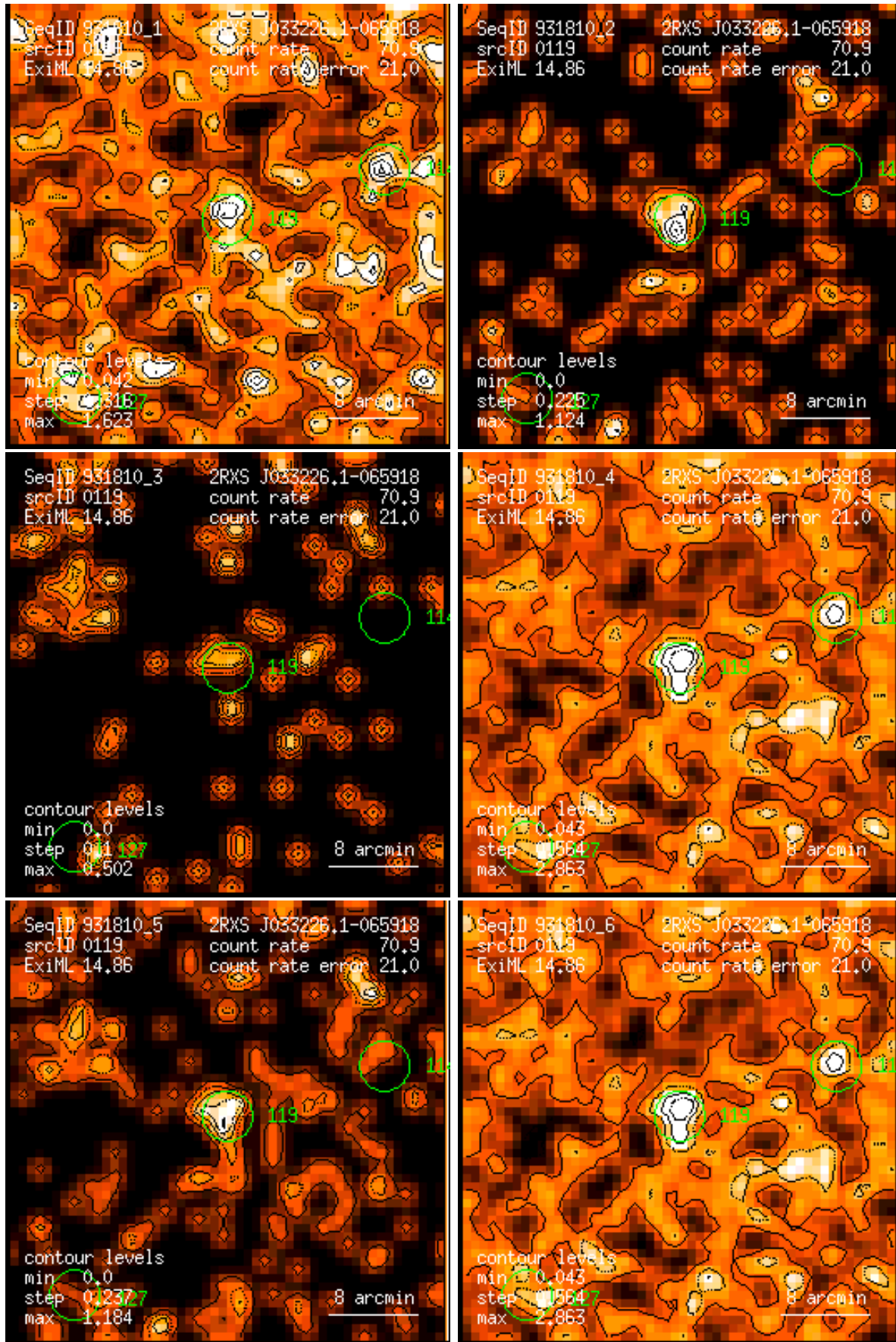
Figure 119: RASS 931810: detection 0119: band rate images, Gaussian filter: (1) PSPC channels 11 – 41, (2) 52 – 90, (3) 91 – 201, (4) 11 – 235, (5) 52 – 201, (6) 11 – 201. Broad band rates in counts/ks. Band rate contour levels in counts/ks/arcmin 2 .
