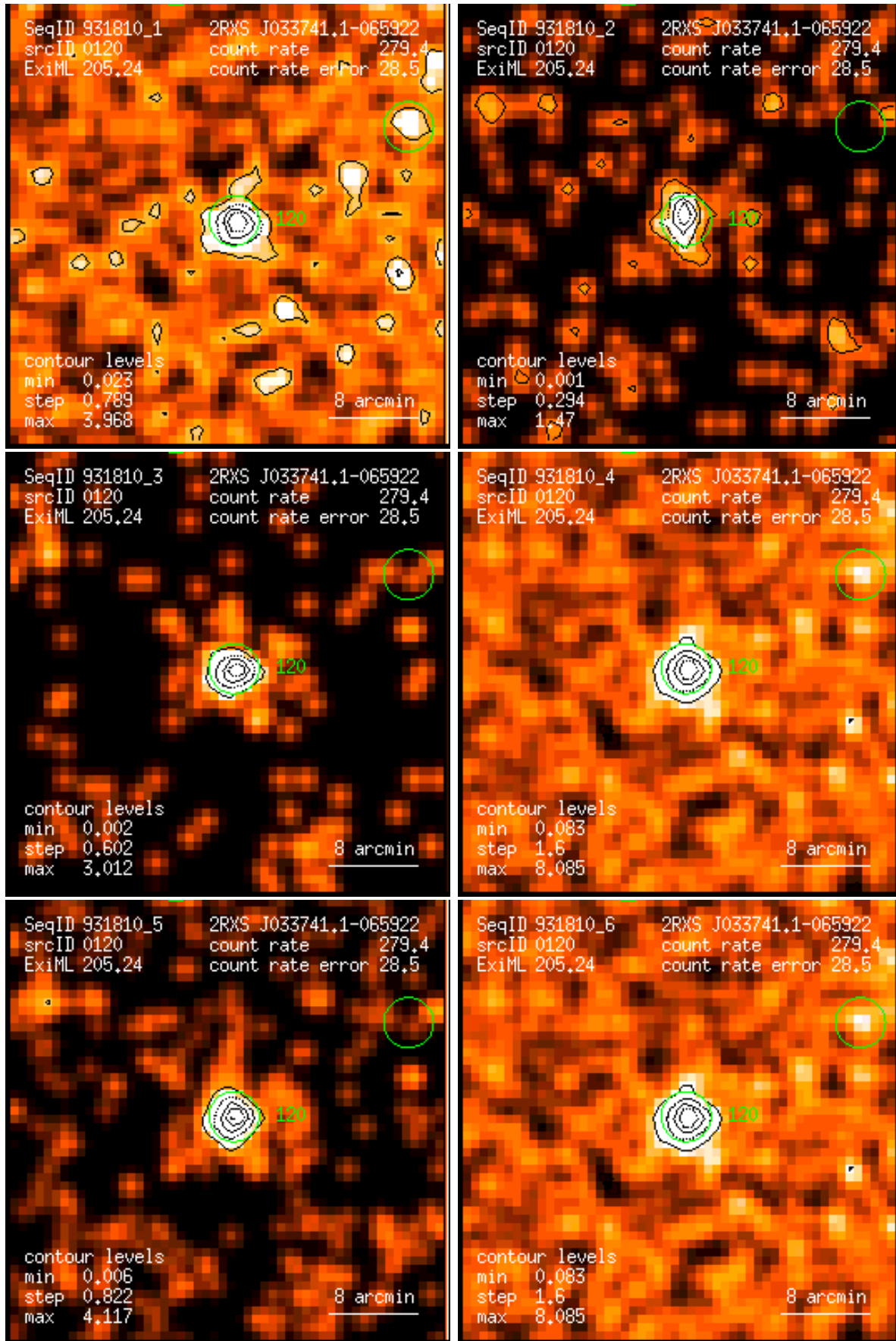
Figure 120: RASS 931810: detection 0120: band rate images, Gaussian filter: (1) PSPC channels 11 – 41, (2) 52 – 90, (3) 91 – 201, (4) 11 – 235, (5) 52 – 201, (6) 11 – 201. Broad band rates in counts/ks. Band rate contour levels in counts/ks/arcmin 2 .
