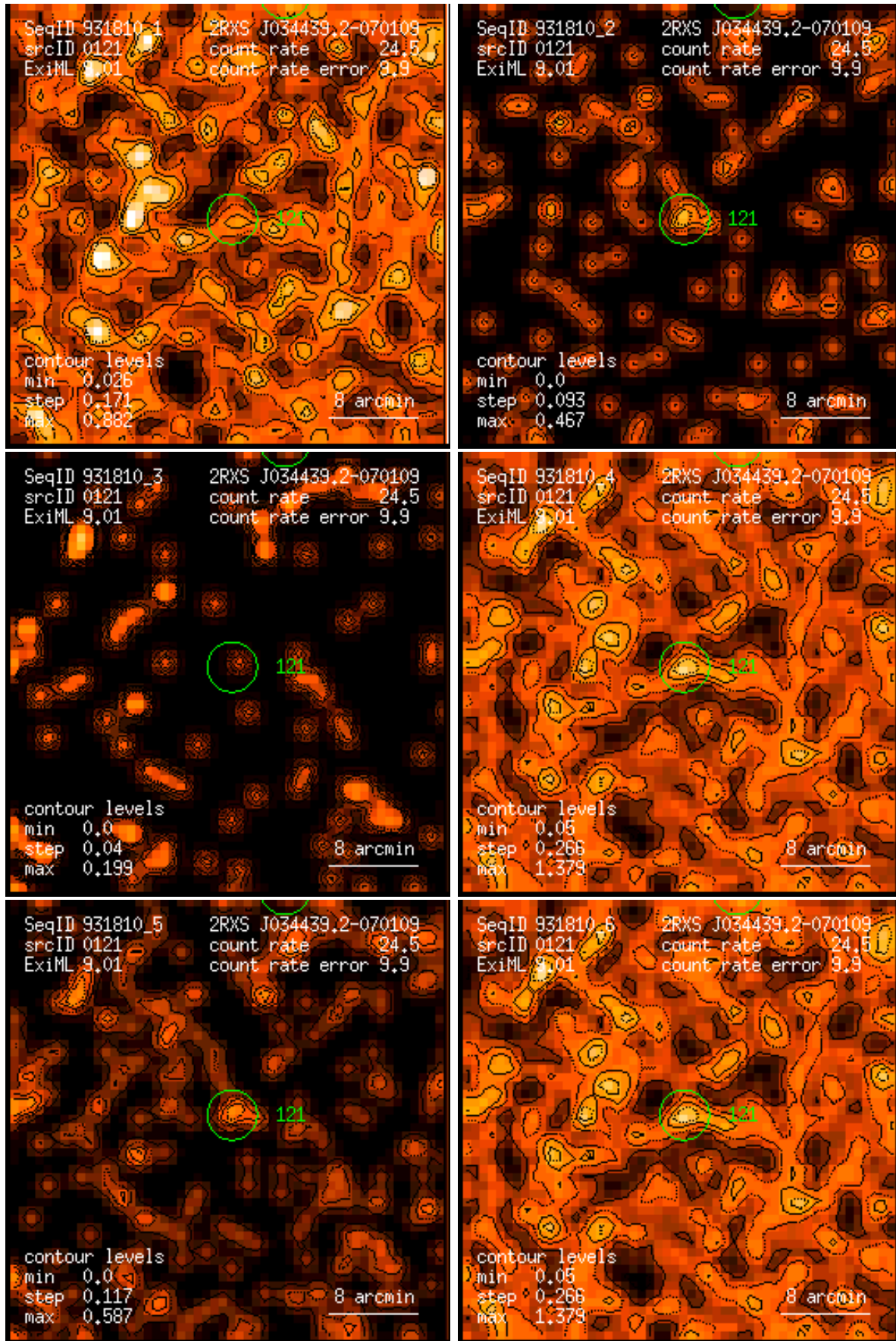
Figure 121: RASS 931810: detection 0121: band rate images, Gaussian filter: (1) PSPC channels 11 – 41, (2) 52 – 90, (3) 91 – 201, (4) 11 – 235, (5) 52 – 201, (6) 11 – 201. Broad band rates in counts/ks. Band rate contour levels in counts/ks/arcmin 2 .
