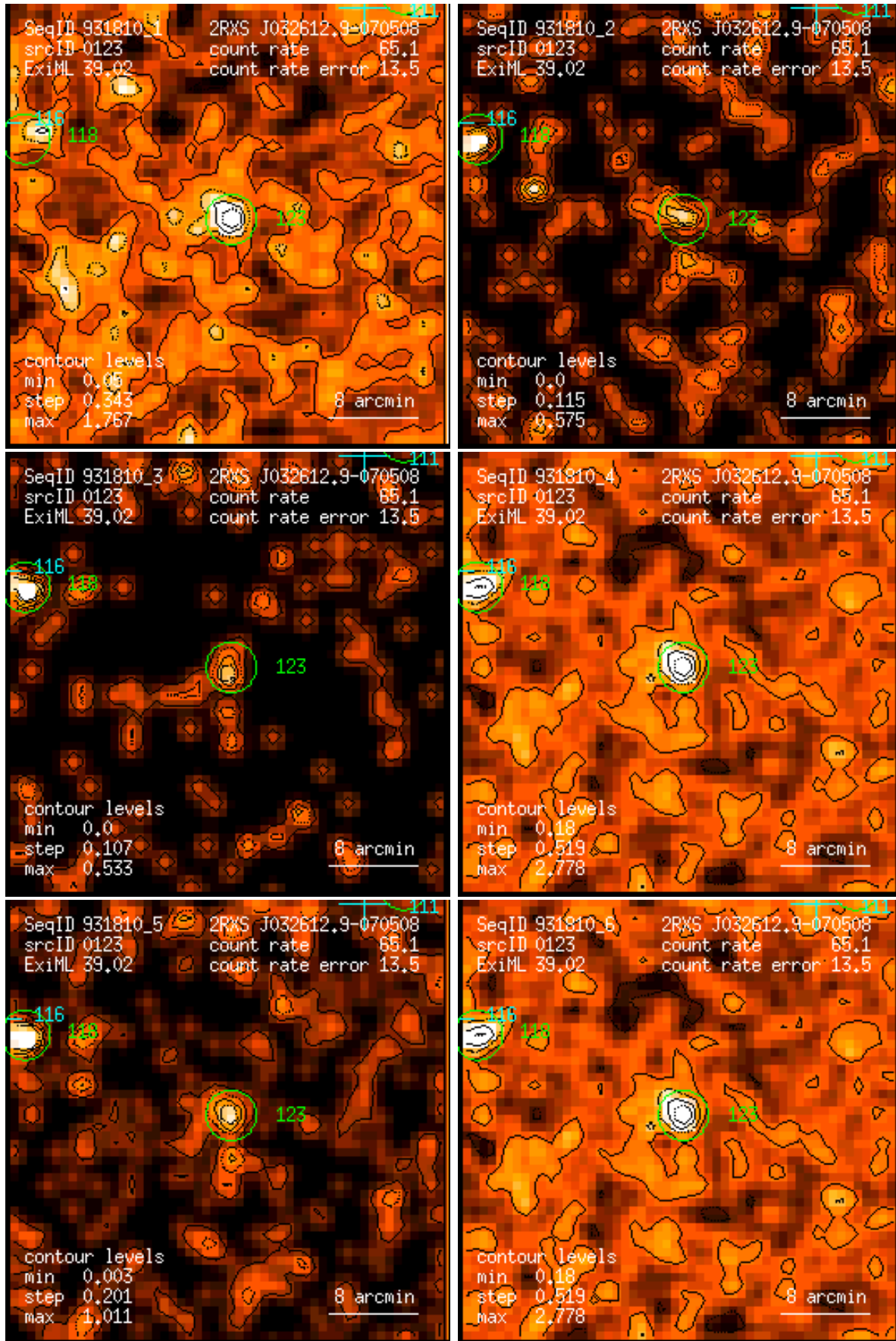
Figure 123: RASS 931810: detection 0123: band rate images, Gaussian filter: (1) PSPC channels 11 – 41, (2) 52 – 90, (3) 91 – 201, (4) 11 – 235, (5) 52 – 201, (6) 11 – 201. Broad band rates in counts/ks. Band rate contour levels in counts/ks/arcmin 2 .
