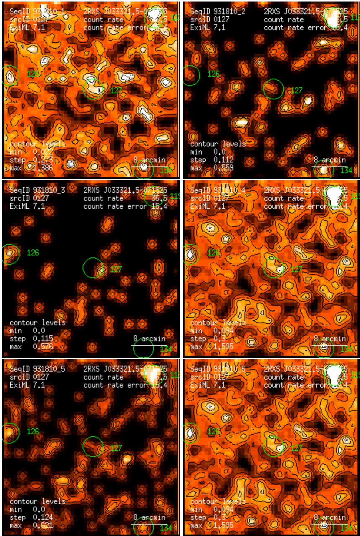
Figure 127: RASS 931810: detection 0127: band rate images, Gaussian filter: (1) PSPC channels 11 – 41, (2) 52 – 90, (3) 91 – 201, (4) 11 – 235, (5) 52 – 201, (6) 11 – 201. Broad band rates in counts/ks. Band rate contour levels in counts/ks/arcmin 2 .
