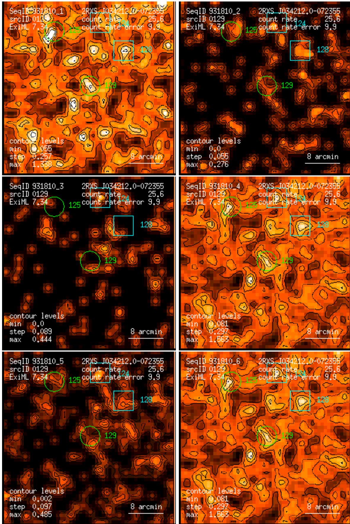
Figure 129: RASS 931810: detection 0129: band rate images, Gaussian filter: (1) PSPC channels 11 – 41, (2) 52 – 90, (3) 91 – 201, (4) 11 – 235, (5) 52 – 201, (6) 11 – 201. Broad band rates in counts/ks. Band rate contour levels in counts/ks/arcmin 2 .
