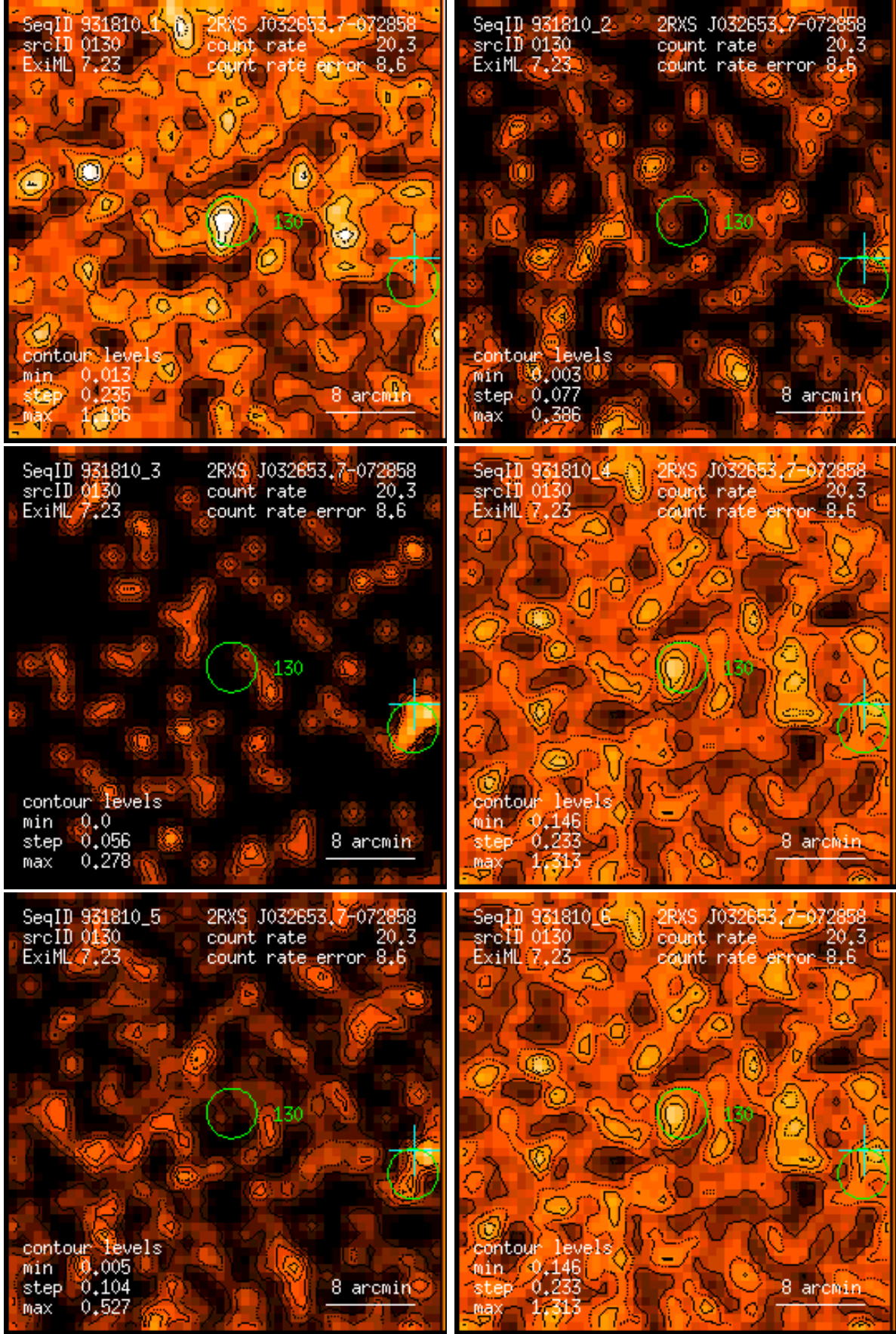
Figure 130: RASS 931810: detection 0130: band rate images, Gaussian filter: (1) PSPC channels 11 – 41, (2) 52 – 90, (3) 91 – 201, (4) 11 – 235, (5) 52 – 201, (6) 11 – 201. Broad band rates in counts/ks. Band rate contour levels in counts/ks/arcmin 2 .
