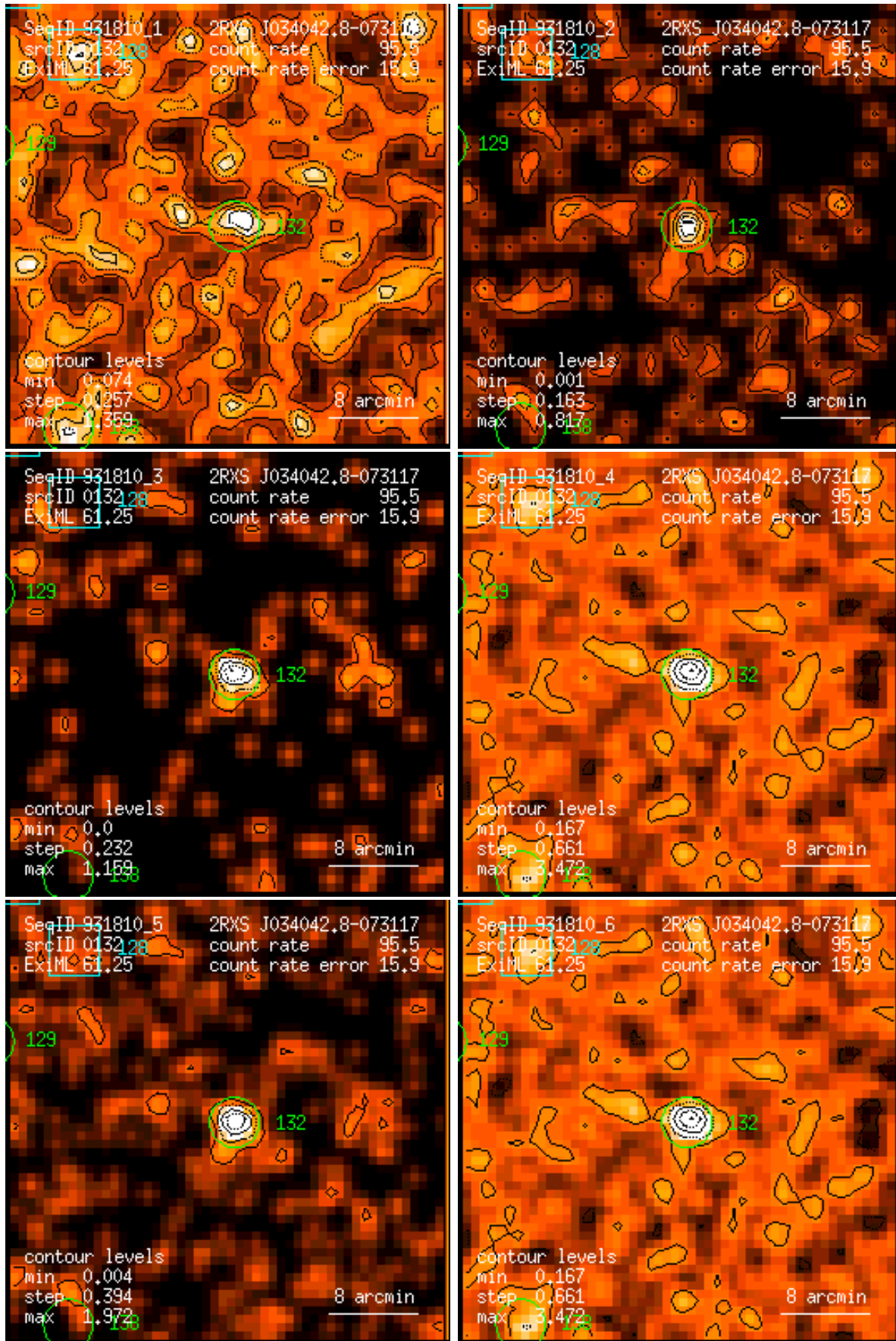
Figure 132: RASS 931810: detection 0132: band rate images, Gaussian filter: (1) PSPC channels 11 – 41, (2) 52 – 90, (3) 91 – 201, (4) 11 – 235, (5) 52 – 201, (6) 11 – 201. Broad band rates in counts/ks. Band rate contour levels in counts/ks/arcmin 2 .
