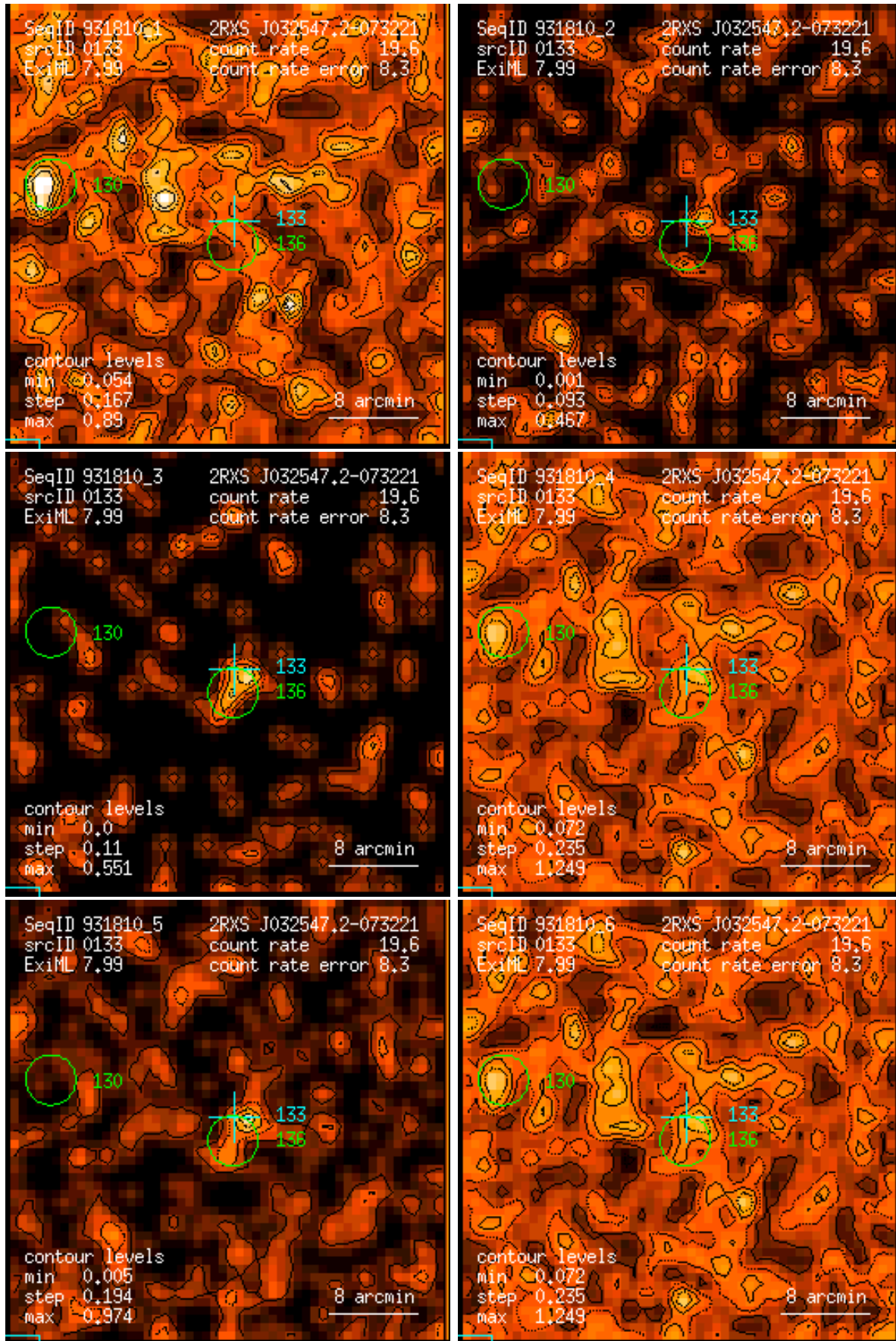
Figure 133: RASS 931810: detection 0133: band rate images, Gaussian filter: (1) PSPC channels 11 – 41, (2) 52 – 90, (3) 91 – 201, (4) 11 – 235, (5) 52 – 201, (6) 11 – 201. Broad band rates in counts/ks. Band rate contour levels in counts/ks/arcmin 2 .
