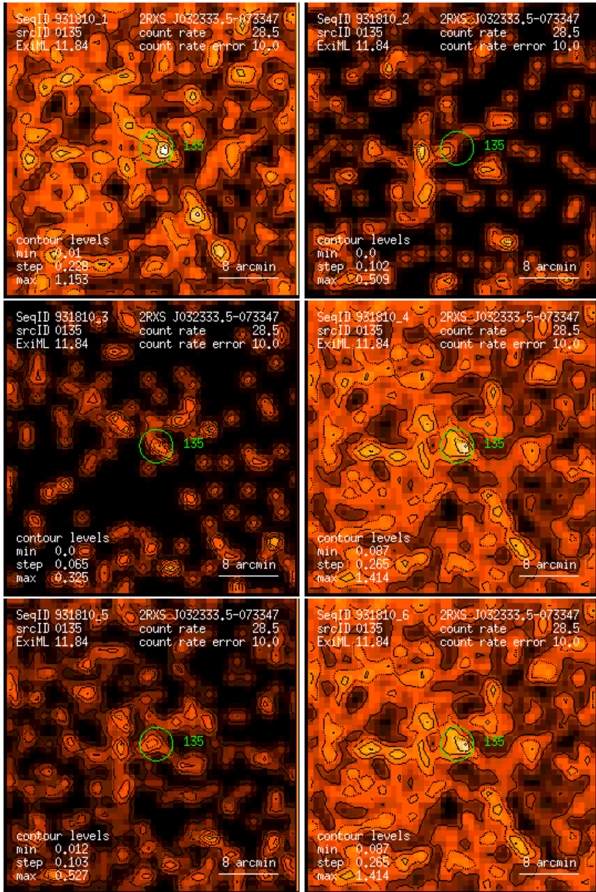
Figure 135: RASS 931810: detection 0135: band rate images, Gaussian filter: (1) PSPC channels 11 – 41, (2) 52 – 90, (3) 91 – 201, (4) 11 – 235, (5) 52 – 201, (6) 11 – 201. Broad band rates in counts/ks. Band rate contour levels in counts/ks/arcmin 2 .
