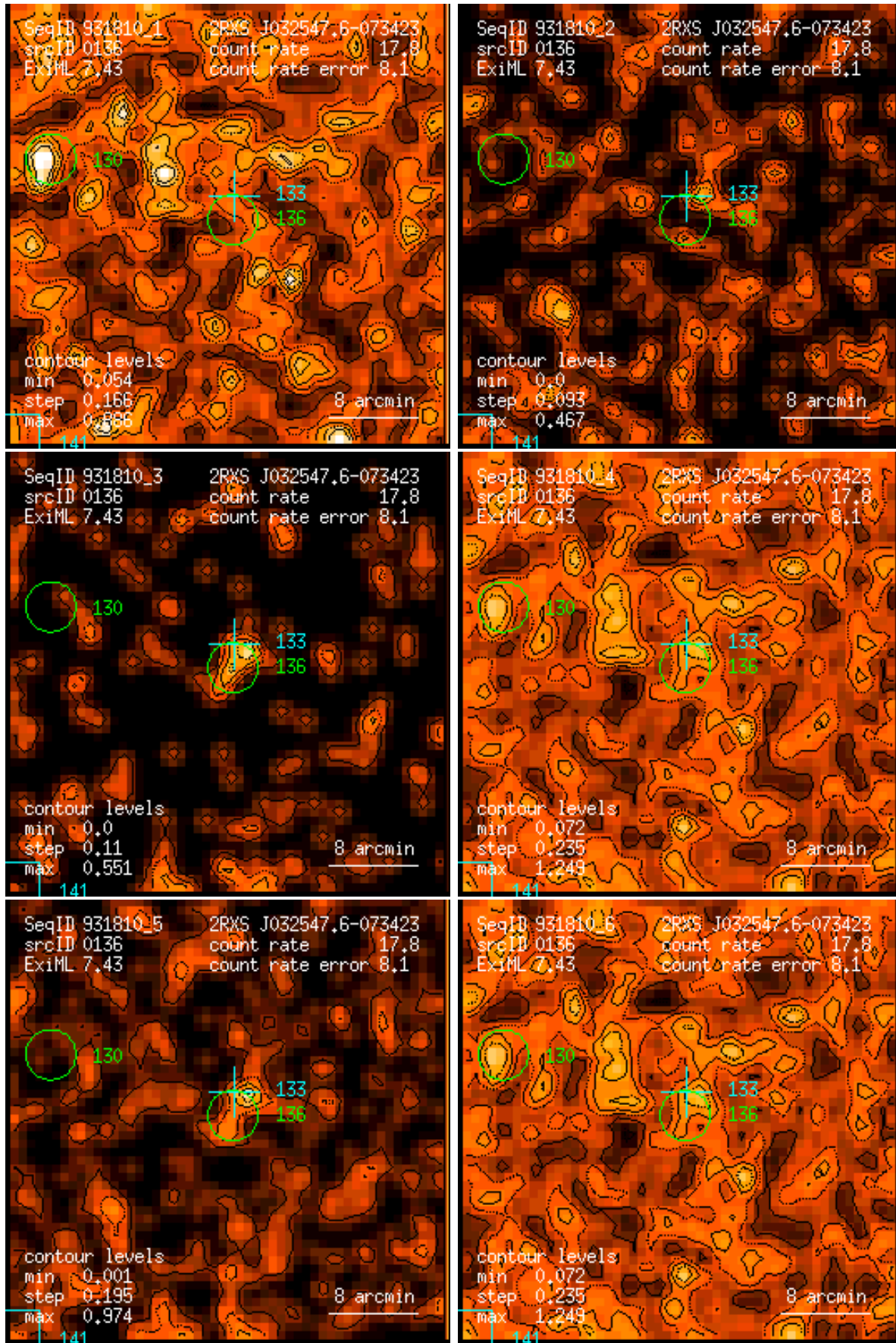
Figure 136: RASS 931810: detection 0136: band rate images, Gaussian filter: (1) PSPC channels 11 – 41, (2) 52 – 90, (3) 91 – 201, (4) 11 – 235, (5) 52 – 201, (6) 11 – 201. Broad band rates in counts/ks. Band rate contour levels in counts/ks/arcmin 2 .
