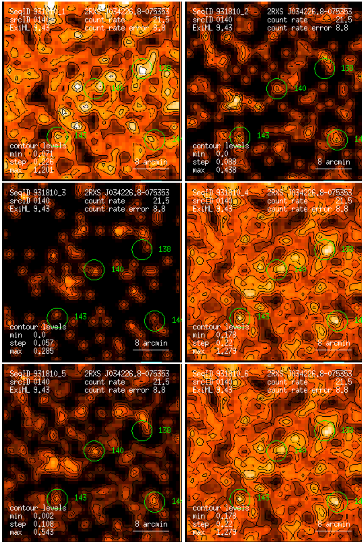
Figure 140: RASS 931810: detection 0140: band rate images, Gaussian filter: (1) PSPC channels 11 – 41, (2) 52 – 90, (3) 91 – 201, (4) 11 – 235, (5) 52 – 201, (6) 11 – 201. Broad band rates in counts/ks. Band rate contour levels in counts/ks/arcmin 2 .
