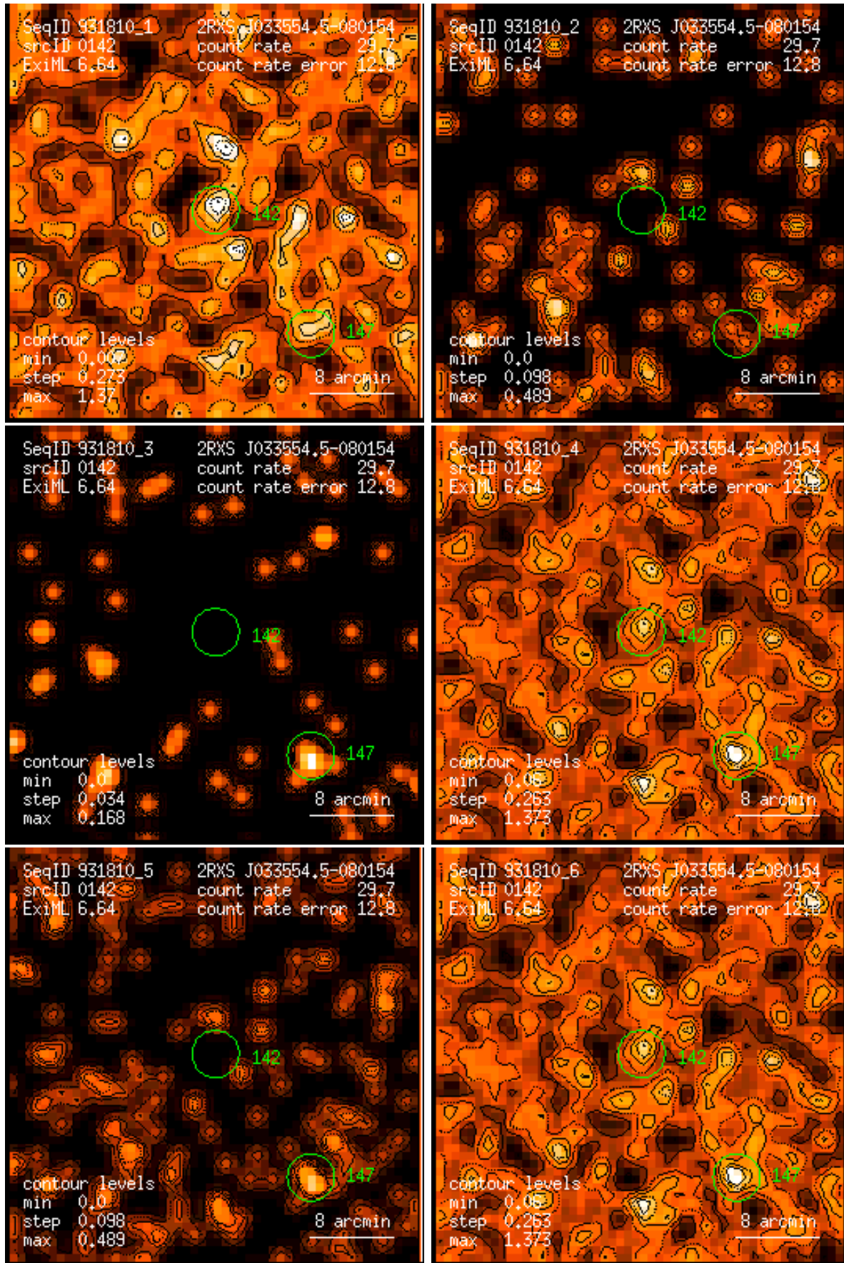
Figure 142: RASS 931810: detection 0142: band rate images, Gaussian filter: (1) PSPC channels 11 – 41, (2) 52 – 90, (3) 91 – 201, (4) 11 – 235, (5) 52 – 201, (6) 11 – 201. Broad band rates in counts/ks. Band rate contour levels in counts/ks/arcmin 2 .
