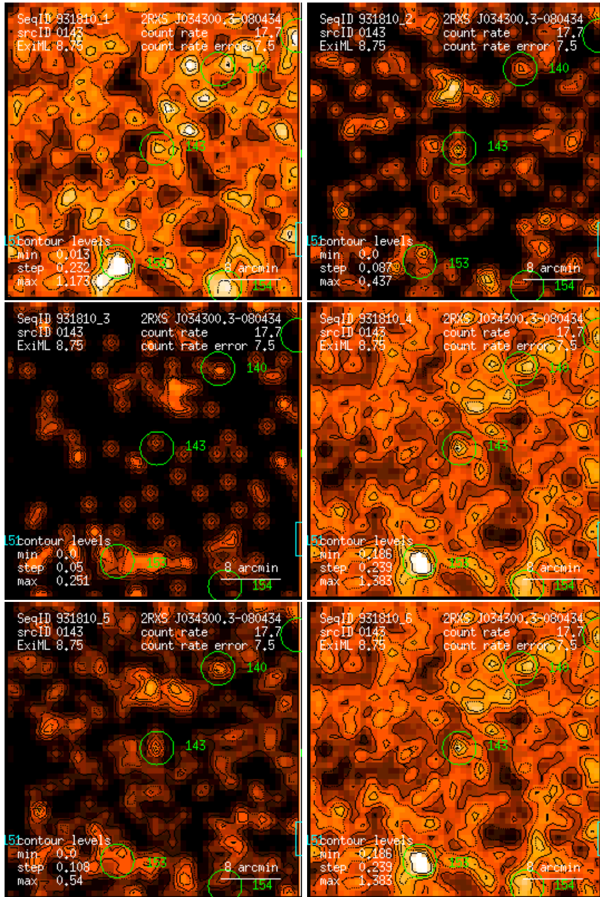
Figure 143: RASS 931810: detection 0143: band rate images, Gaussian filter: (1) PSPC channels 11 – 41, (2) 52 – 90, (3) 91 – 201, (4) 11 – 235, (5) 52 – 201, (6) 11 – 201. Broad band rates in counts/ks. Band rate contour levels in counts/ks/arcmin 2 .
