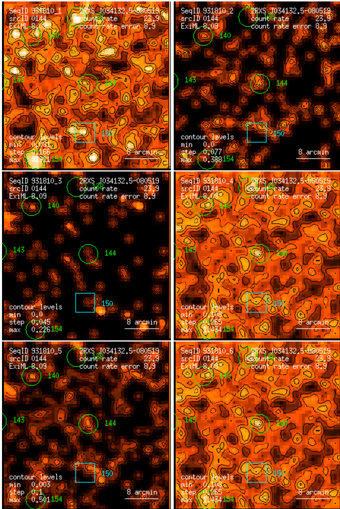
Figure 144: RASS 931810: detection 0144: band rate images, Gaussian filter: (1) PSPC channels 11 – 41, (2) 52 – 90, (3) 91 – 201, (4) 11 – 235, (5) 52 – 201, (6) 11 – 201. Broad band rates in counts/ks. Band rate contour levels in counts/ks/arcmin 2 .
