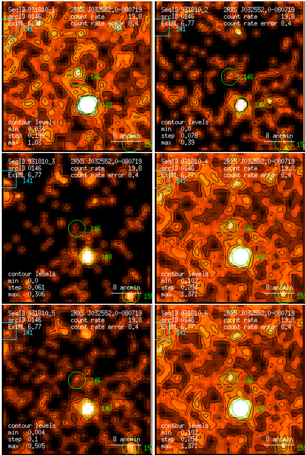
Figure 146: RASS 931810: detection 0146: band rate images, Gaussian filter: (1) PSPC channels 11 – 41, (2) 52 – 90, (3) 91 – 201, (4) 11 – 235, (5) 52 – 201, (6) 11 – 201. Broad band rates in counts/ks. Band rate contour levels in counts/ks/arcmin 2 .
