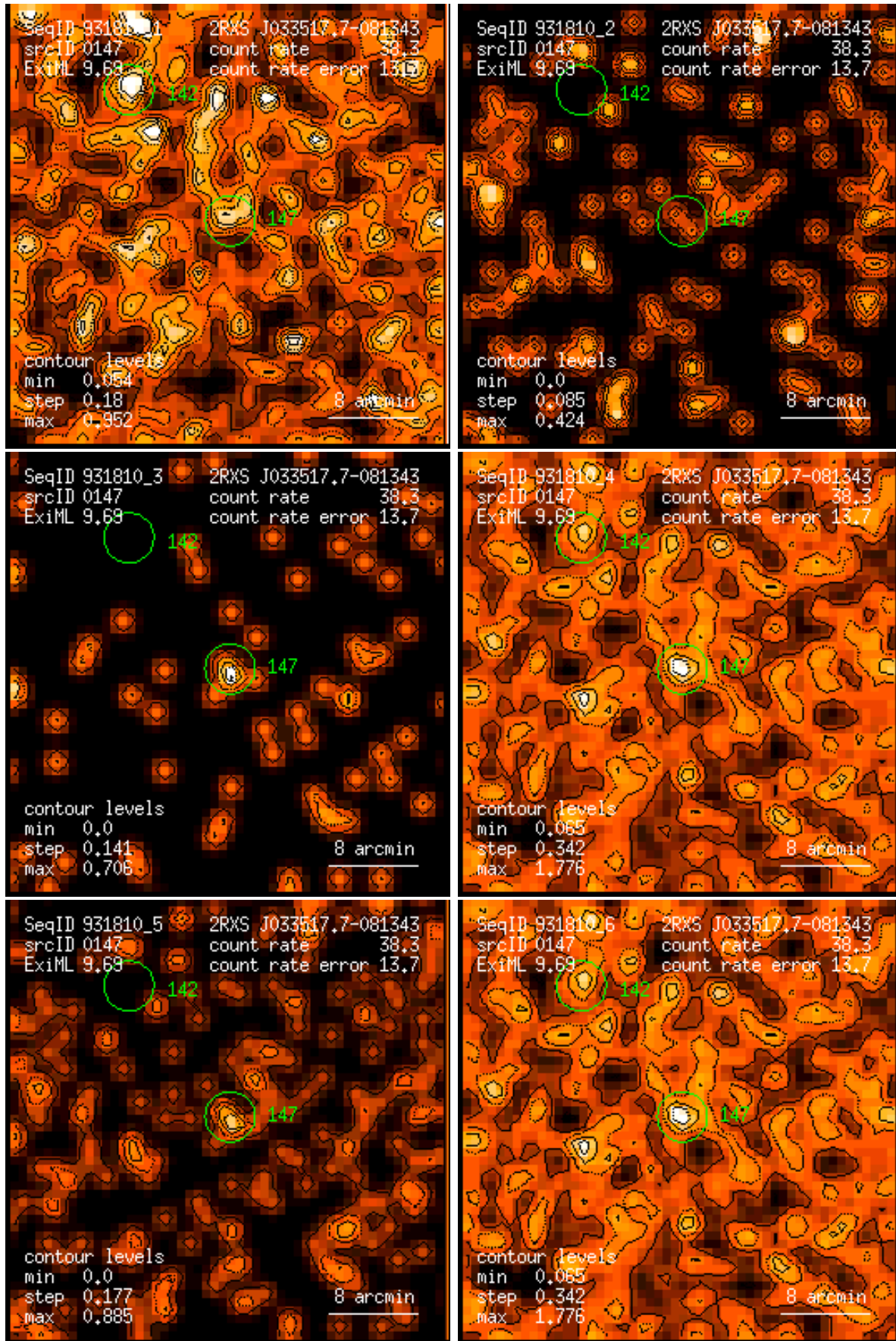
Figure 147: RASS 931810: detection 0147: band rate images, Gaussian filter: (1) PSPC channels 11 – 41, (2) 52 – 90, (3) 91 – 201, (4) 11 – 235, (5) 52 – 201, (6) 11 – 201. Broad band rates in counts/ks. Band rate contour levels in counts/ks/arcmin 2 .
