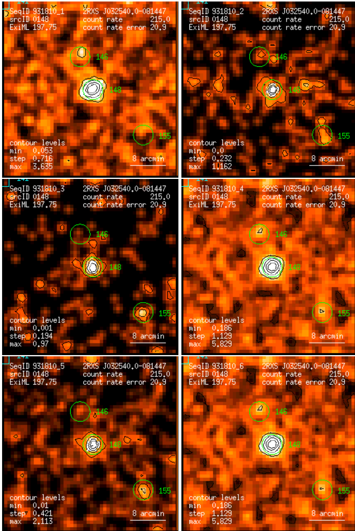
Figure 148: RASS 931810: detection 0148: band rate images, Gaussian filter: (1) PSPC channels 11 – 41, (2) 52 – 90, (3) 91 – 201, (4) 11 – 235, (5) 52 – 201, (6) 11 – 201. Broad band rates in counts/ks. Band rate contour levels in counts/ks/arcmin 2 .
