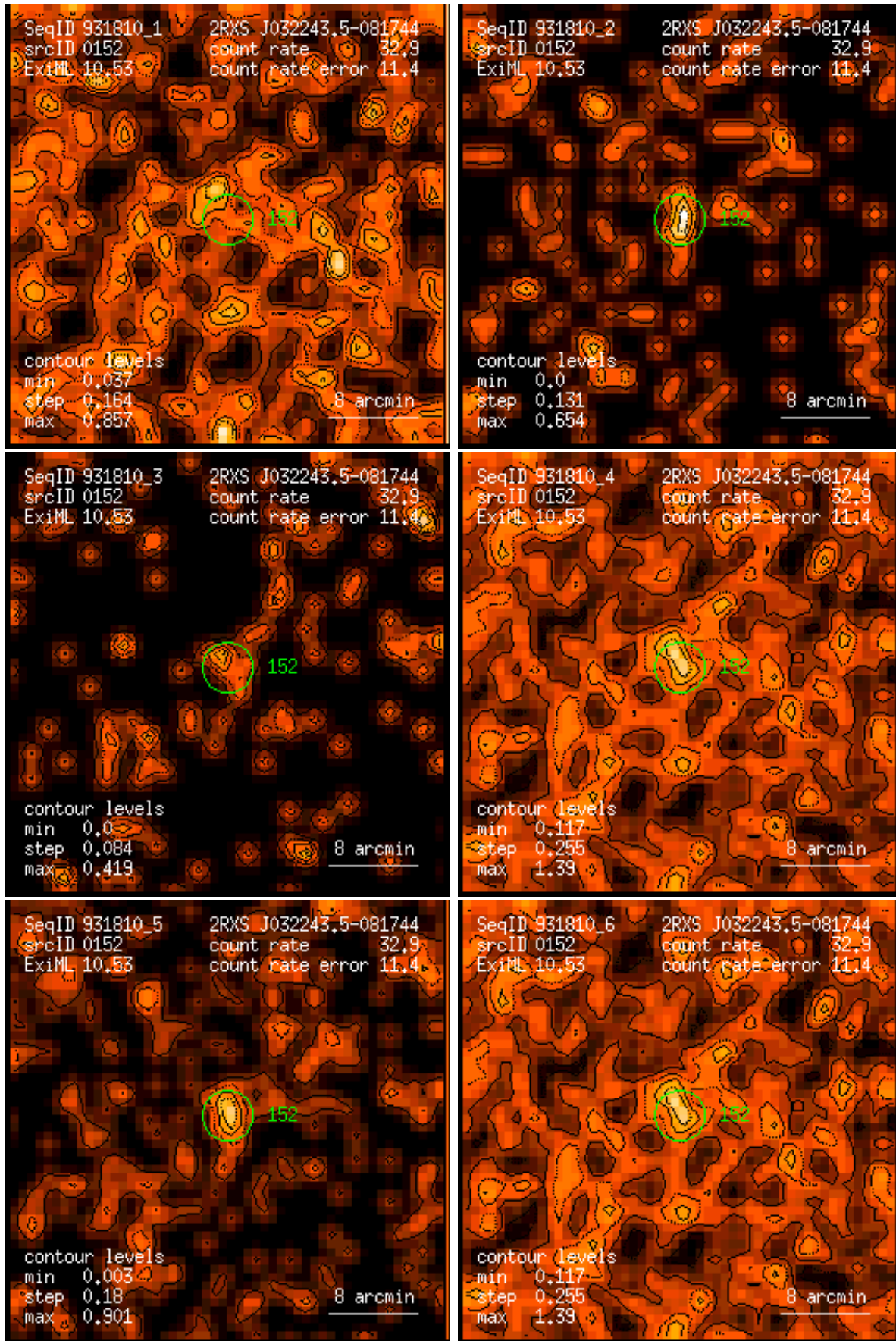
Figure 152: RASS 931810: detection 0152: band rate images, Gaussian filter: (1) PSPC channels 11 – 41, (2) 52 – 90, (3) 91 – 201, (4) 11 – 235, (5) 52 – 201, (6) 11 – 201. Broad band rates in counts/ks. Band rate contour levels in counts/ks/arcmin 2 .
