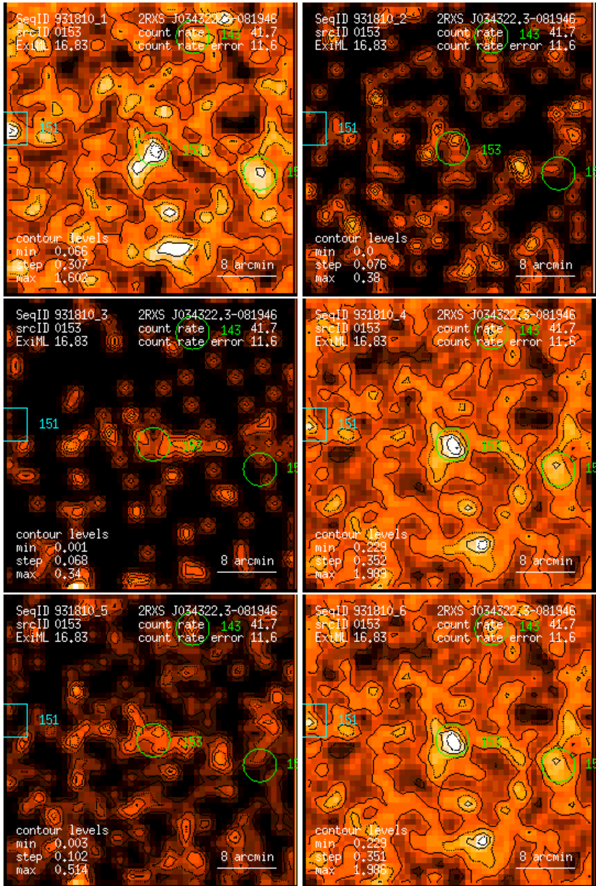
Figure 153: RASS 931810: detection 0153: band rate images, Gaussian filter: (1) PSPC channels 11 – 41, (2) 52 – 90, (3) 91 – 201, (4) 11 – 235, (5) 52 – 201, (6) 11 – 201. Broad band rates in counts/ks. Band rate contour levels in counts/ks/arcmin 2 .
