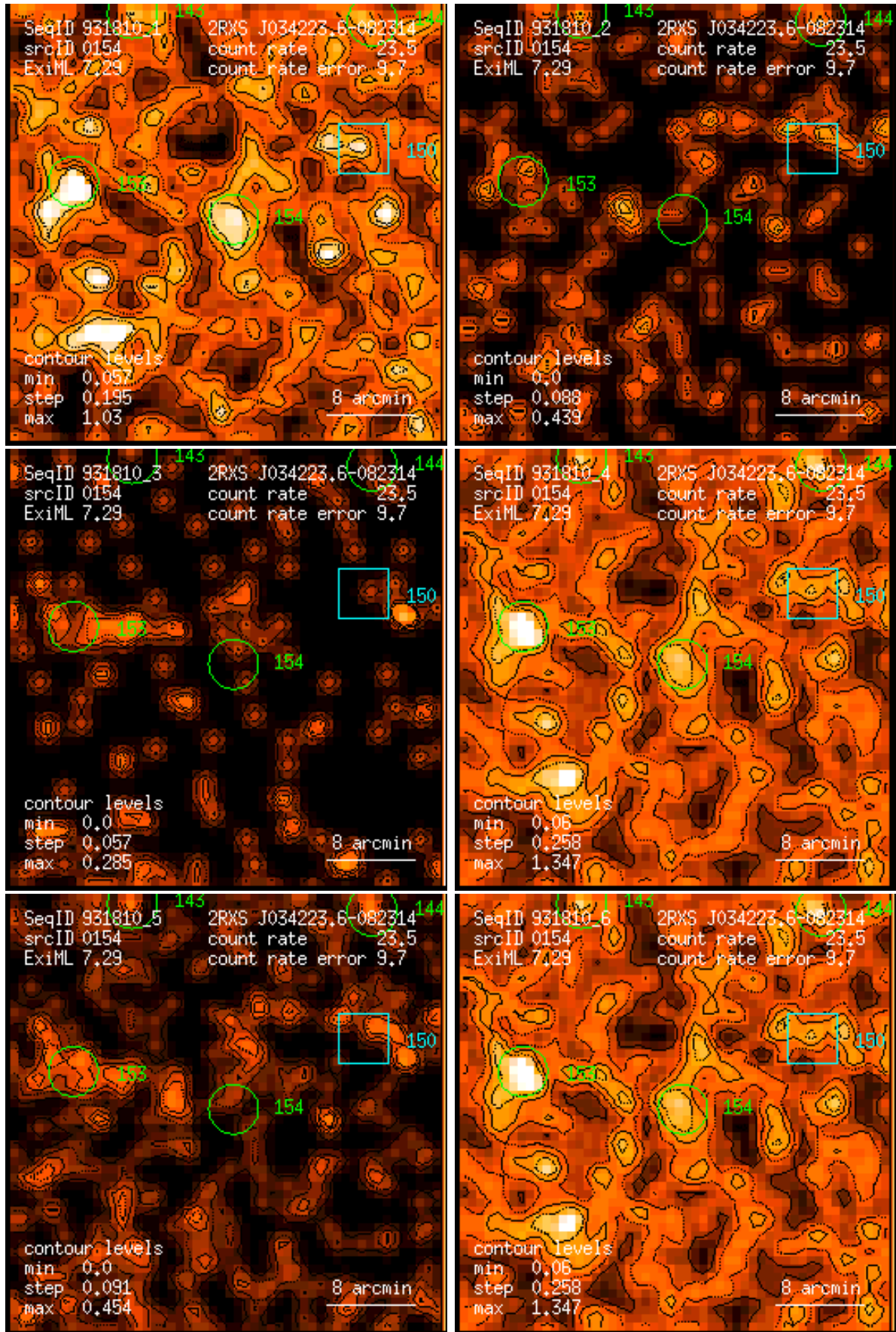
Figure 154: RASS 931810: detection 0154: band rate images, Gaussian filter: (1) PSPC channels 11 – 41, (2) 52 – 90, (3) 91 – 201, (4) 11 – 235, (5) 52 – 201, (6) 11 – 201. Broad band rates in counts/ks. Band rate contour levels in counts/ks/arcmin 2 .
