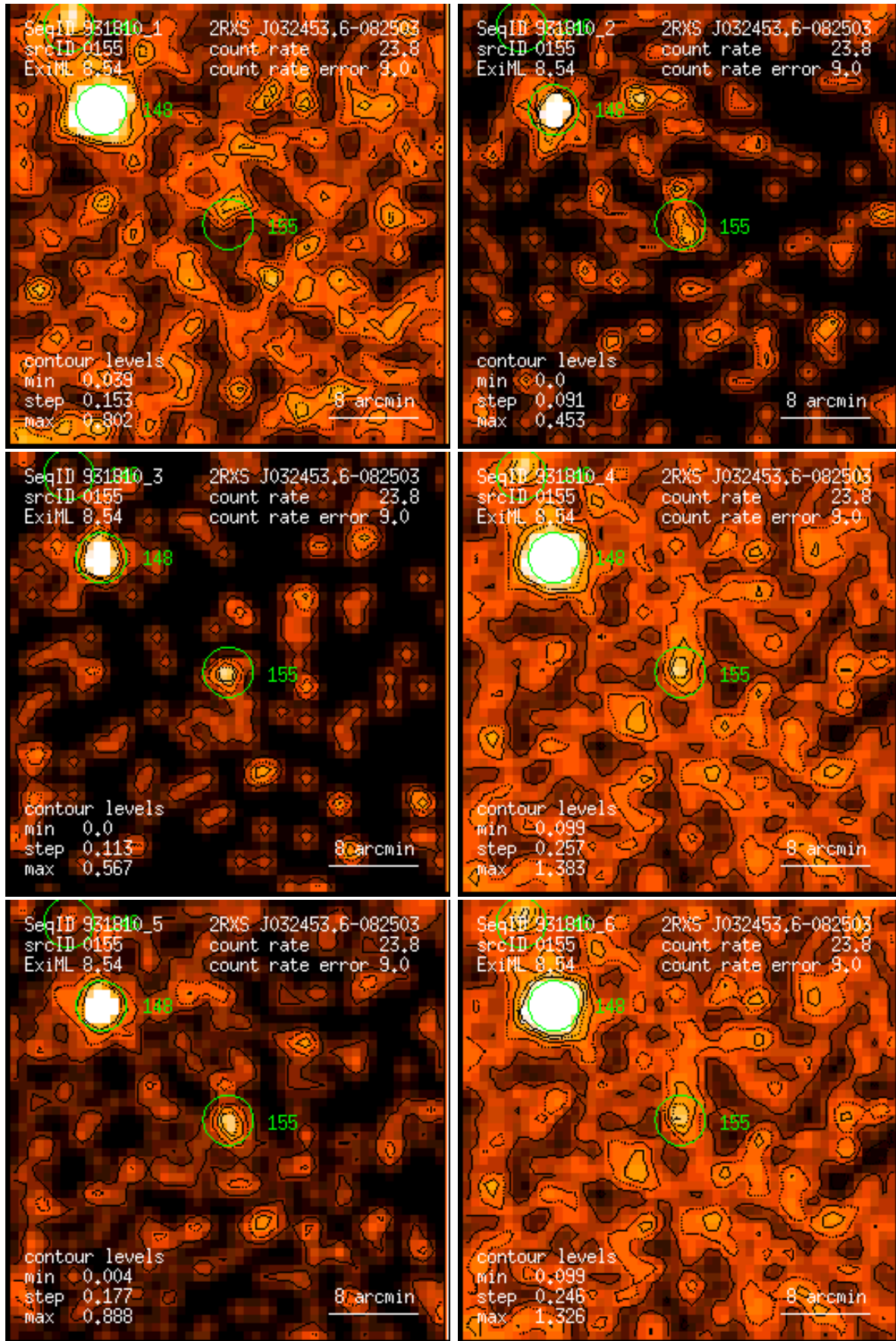
Figure 155: RASS 931810: detection 0155: band rate images, Gaussian filter: (1) PSPC channels 11 – 41, (2) 52 – 90, (3) 91 – 201, (4) 11 – 235, (5) 52 – 201, (6) 11 – 201. Broad band rates in counts/ks. Band rate contour levels in counts/ks/arcmin 2 .
