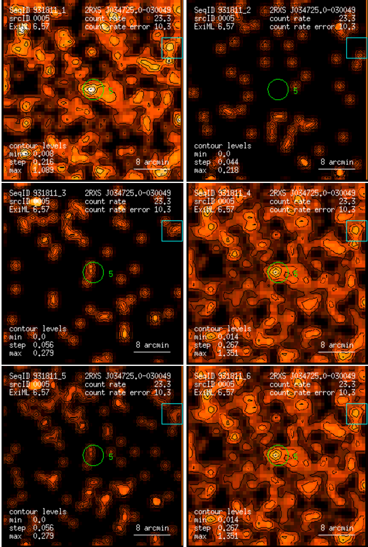
Figure 5: RASS 931811: detection 0005: band rate images, Gaussian filter: (1) PSPC channels 11 – 41, (2) 52 – 90, (3) 91 – 201, (4) 11 – 235, (5) 52 – 201, (6) 11 – 201. Broad band rates in counts/ks. Band rate contour levels in counts/ks/arcmin 2 .
