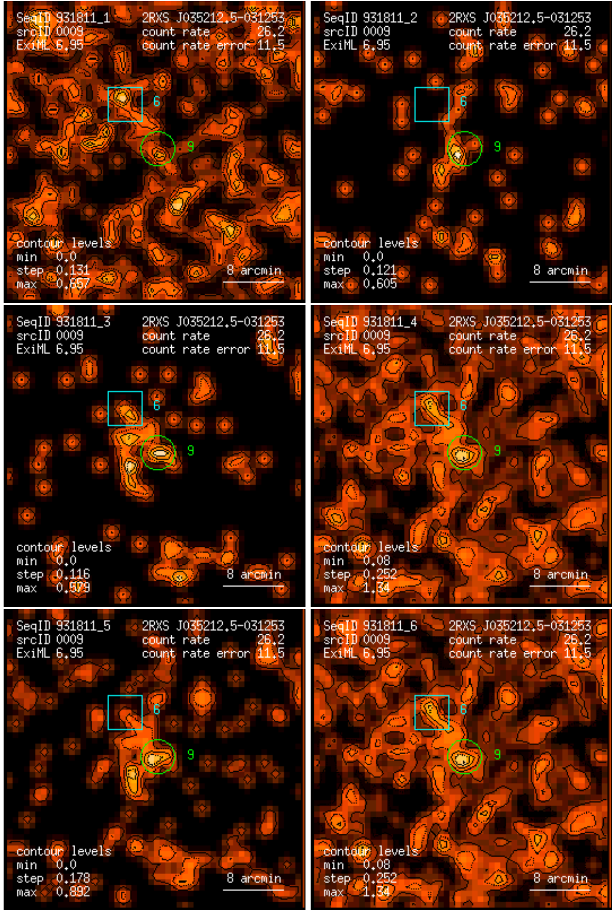
Figure 9: RASS 931811: detection 0009: band rate images, Gaussian filter: (1) PSPC channels 11 – 41, (2) 52 – 90, (3) 91 – 201, (4) 11 – 235, (5) 52 – 201, (6) 11 – 201. Broad band rates in counts/ks. Band rate contour levels in counts/ks/arcmin 2 .
