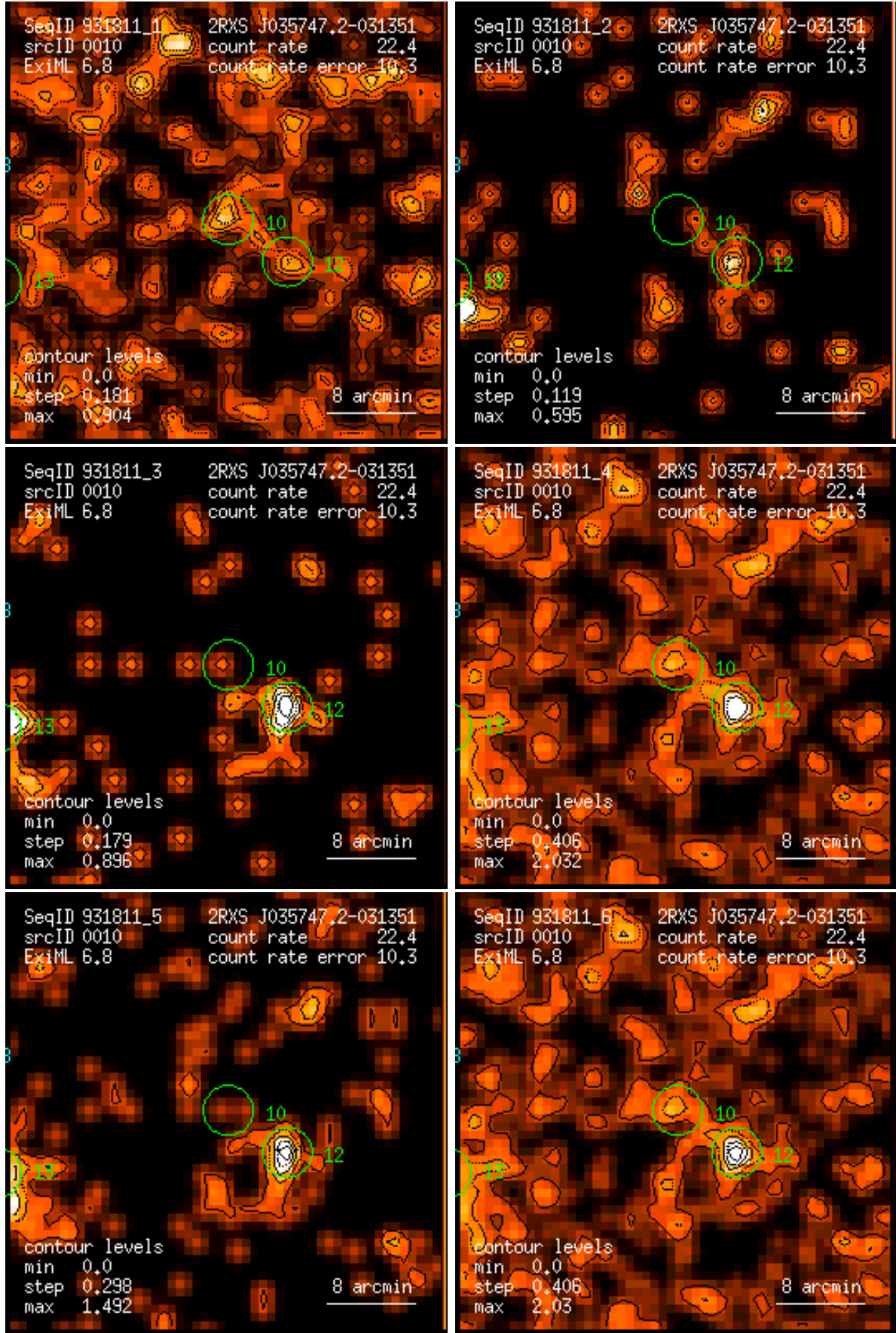
Figure 10: RASS 931811: detection 0010: band rate images, Gaussian filter: (1) PSPC channels 11 – 41, (2) 52 – 90, (3) 91 – 201, (4) 11 – 235, (5) 52 – 201, (6) 11 – 201. Broad band rates in counts/ks. Band rate contour levels in counts/ks/arcmin 2 .
