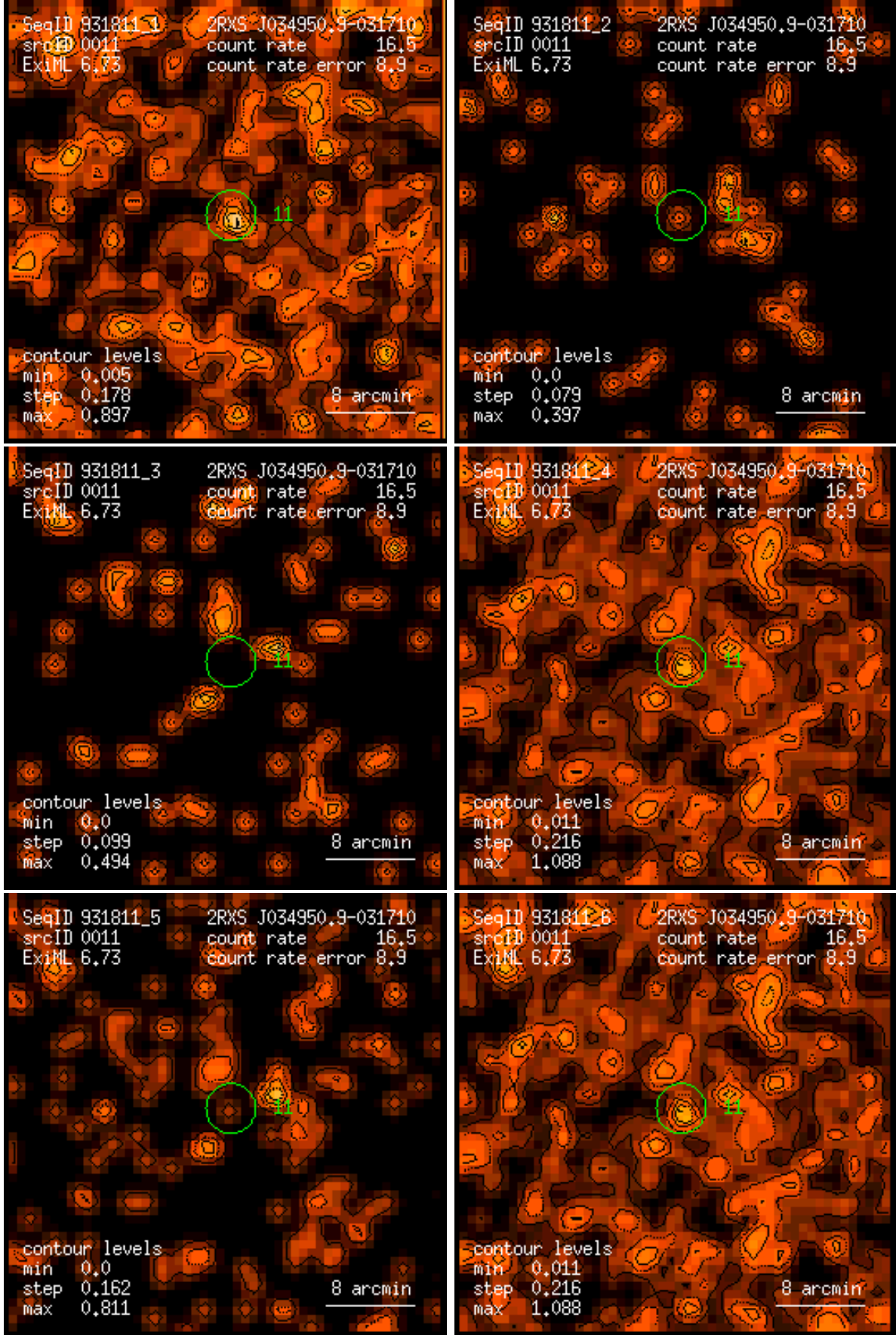
Figure 11: RASS 931811: detection 0011: band rate images, Gaussian filter: (1) PSPC channels 11 – 41, (2) 52 – 90, (3) 91 – 201, (4) 11 – 235, (5) 52 – 201, (6) 11 – 201. Broad band rates in counts/ks. Band rate contour levels in counts/ks/arcmin 2 .
