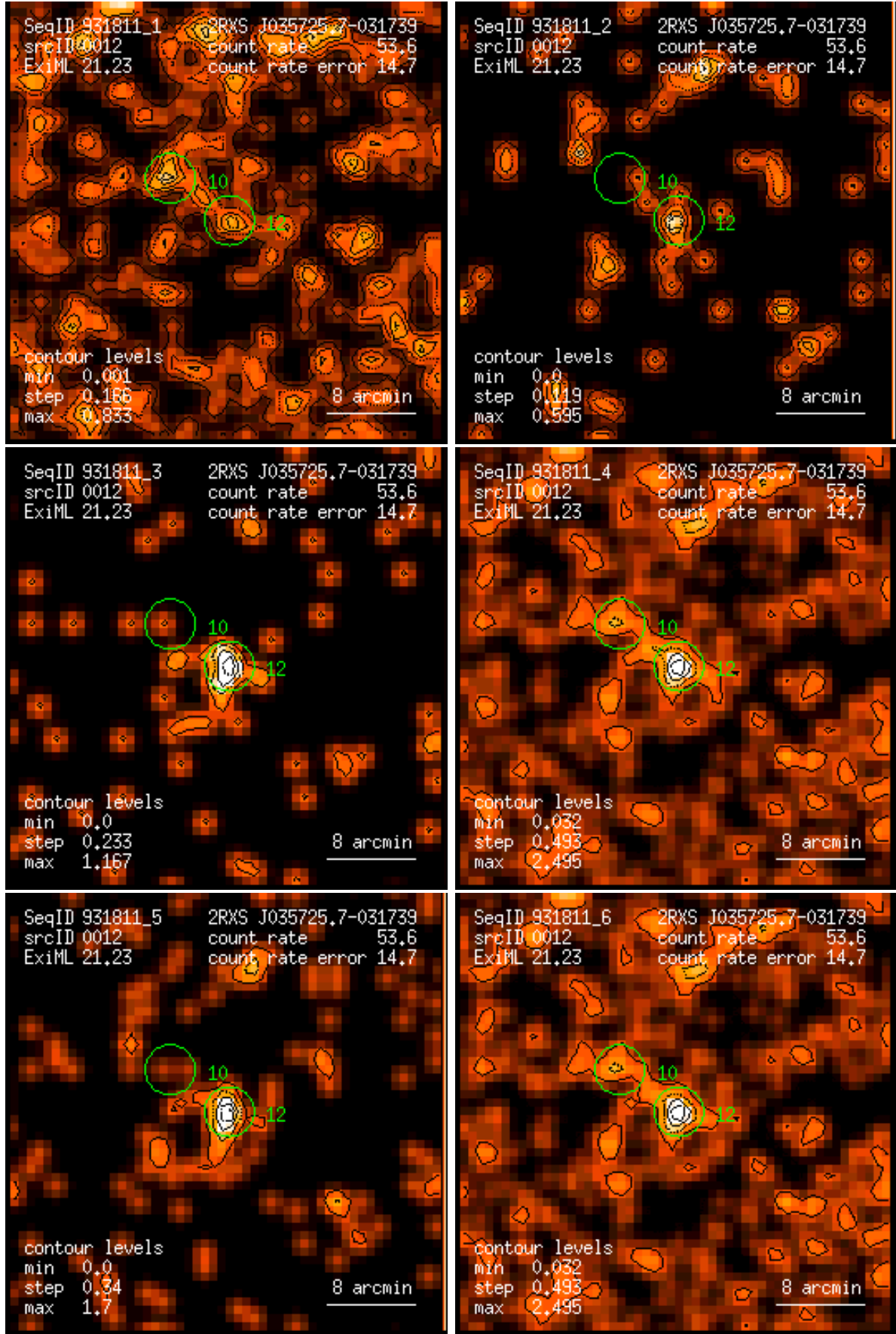
Figure 12: RASS 931811: detection 0012: band rate images, Gaussian filter: (1) PSPC channels 11 – 41, (2) 52 – 90, (3) 91 – 201, (4) 11 – 235, (5) 52 – 201, (6) 11 – 201. Broad band rates in counts/ks. Band rate contour levels in counts/ks/arcmin 2 .
