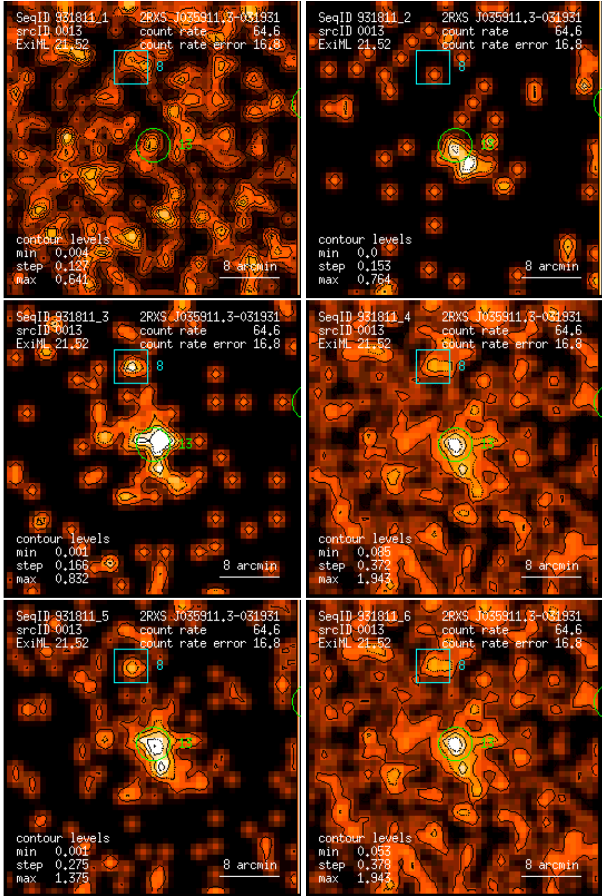
Figure 13: RASS 931811: detection 0013: band rate images, Gaussian filter: (1) PSPC channels 11 – 41, (2) 52 – 90, (3) 91 – 201, (4) 11 – 235, (5) 52 – 201, (6) 11 – 201. Broad band rates in counts/ks. Band rate contour levels in counts/ks/arcmin 2 .
