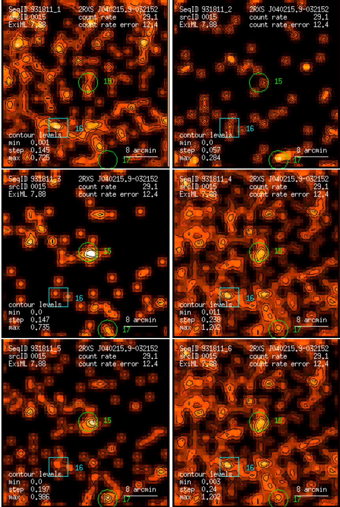
Figure 15: RASS 931811: detection 0015: band rate images, Gaussian filter: (1) PSPC channels 11 – 41, (2) 52 – 90, (3) 91 – 201, (4) 11 – 235, (5) 52 – 201, (6) 11 – 201. Broad band rates in counts/ks. Band rate contour levels in counts/ks/arcmin 2 .
